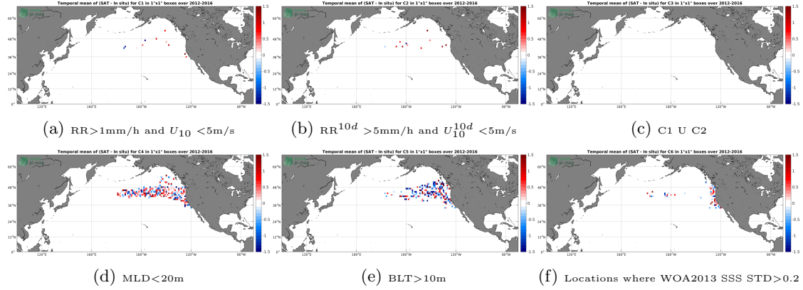
Figure 12: Temporal mean gridded over spatial boxes of size 1^\circ \times 1^\circ of \Delta\text{SSS} (SMOS-L2-DPGS-v662 - Sea mammals) for 6 different subdatasets corresponding to: \text{RR} > 1\text{mm/h} and U_{10} < 5\text{m/s} (a), \text{RR}^{10d} > 5\text{mm/h} and U_{10}^{10d} < 5\text{m/s} (b), C1 U C2 (c), \text{MLD} < 20\text{m} (d), \text{BLT} > 10\text{m} (e), Locations where WOA2013 SSS STD > 0.2 (f).
