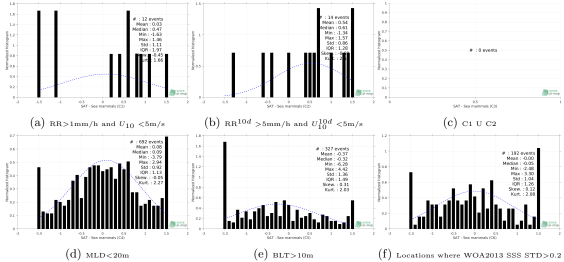
Figure 13: Normalized histogram of \Delta\text{SSS} (SMOS-L2-DPGS-v662 - Sea mammals) for 6 different subdatasets corresponding to: \text{RR} > 1\text{mm/h} and U_{10} < 5\text{m/s} (a), \text{RR}^{10d} > 5\text{mm/h} and U_{10}^{10d} < 5\text{m/s} (b), C1 U C2 (c), \text{MLD} < 20\text{m} (d), \text{BLT} > 10\text{m} (e), Locations where WOA2013 SSS STD > 0.2 (f).
