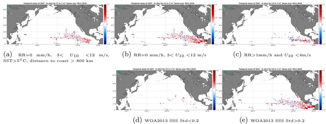
Figure 11: Temporal mean gridded over spatial boxes of size 1^\circ \times 1^\circ of \Delta SSS (SMOS SSS L2 v662 (ESA) - Surface drifters) for 5 different subdatasets corresponding to:RR=0 mm/h, 3 < U_{10} < 12 m/s, SST >5^\circ\text{C} , distance to coast > 800 km (a), RR=0 mm/h, 3 < U_{10} < 12 m/s (b), RR >1 mm/h and U_{10} < 4 m/s (c), WOA2013 SSS Std <0.2 (d), WOA2013 SSS Std >0.2 (e).
