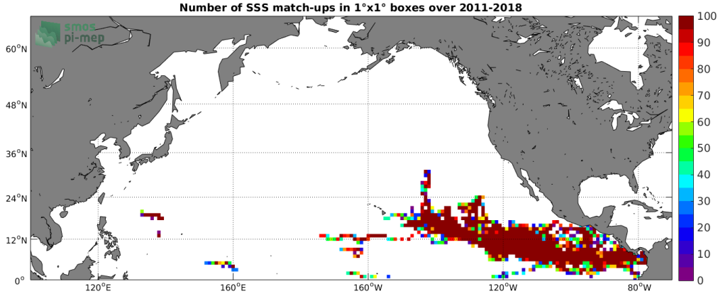
Figure 3: Number of SSS match-ups between Surface drifters SSS and the SMOS SSS L2 v662 (ESA) SSS product for the North Pacific Ocean Pi-MEP region over 1^\circ \times 1^\circ boxes and for the full satellite product period.
