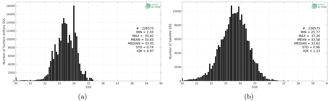
Figure 2: Histograms of SSS from Surface drifters (a) and SMOS SSS L2 v662 (ESA) (b) considering all match-up pairs per bins of 0.1 over the North Pacific Ocean Pi-MEP region and for the full satellite product period.
