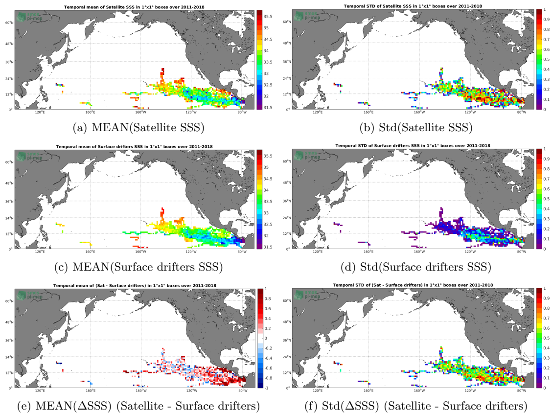
Figure 5: Temporal mean (left) and Std (right) of SSS from SMOS SSS L2 v662 (ESA) (top), Surface drifters (middle), and of \Delta SSS (Satellite - Surface drifters). Only match-up pairs are used to generate these maps.
