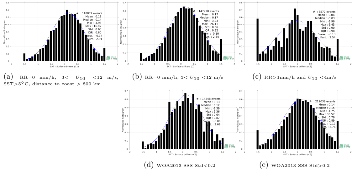
Figure 12: Normalized histogram of \Delta SSS (SMOS SSS L2 v662 (ESA) - Surface drifters) for 5 different subdatasets corresponding to: RR=0 mm/h, 3 < U_{10} < 12 m/s, SST > 5°C, distance to coast > 800 km (a), RR=0 mm/h, 3 < U_{10} < 12 m/s (b), RR > 1mm/h and U_{10} < 4 m/s (c), WOA2013 SSS Std < 0.2 (d), WOA2013 SSS Std > 0.2 (e).
