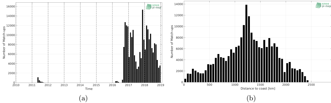
Figure 1: Number of match-ups between Surface drifters and SMOS SSS L2 v662 (ESA) SSS as a function of time (a) and as function of the distance to coast (b) over the North Pacific Ocean Pi-MEP region and for the full satellite product period.
