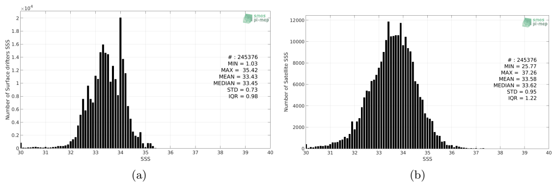
Figure 2: Histograms of SSS from Surface drifters (a) and SMOS SSS L2 v662 (ESA) (b) considering all match-up pairs per bins of 0.1 over the North Pacific Ocean Pi-MEP region and for the full satellite product period.
