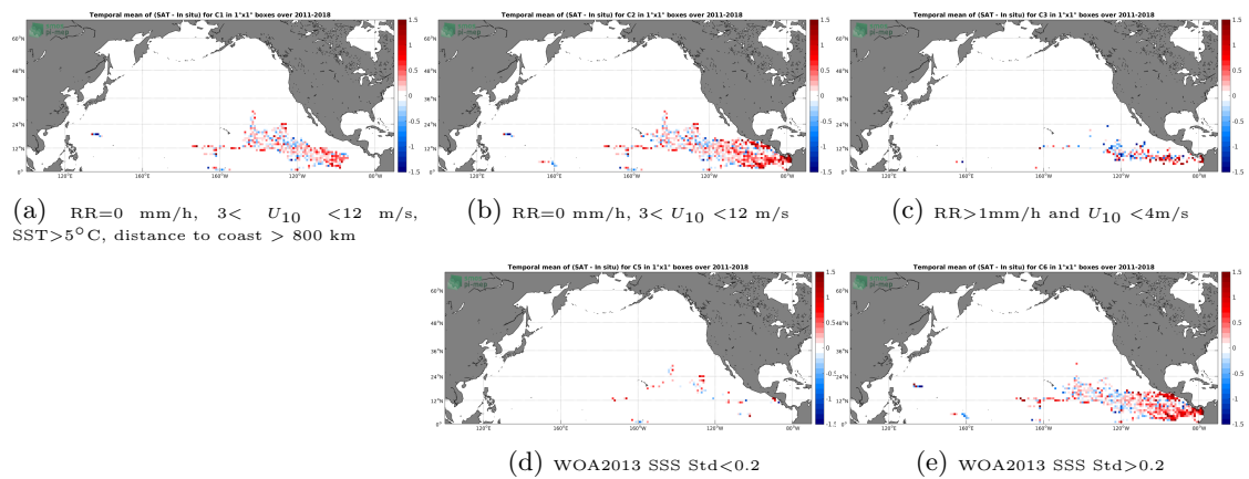
Figure 11: Temporal mean gridded over spatial boxes of size 1°x1° of \Delta SSS (SMOS SSS L2 v662 (ESA) - Surface drifters) for 5 different subdatasets corresponding to:RR=0 mm/h, 3 < U_{10} < 12 m/s, SST>5°C, distance to coast > 800 km (a), RR=0 mm/h, 3 < U_{10} < 12 m/s (b), RR>1mm/h and U_{10} < 4 m/s (c), WOA2013 SSS Std<0.2 (d), WOA2013 SSS Std>0.2 (e).
