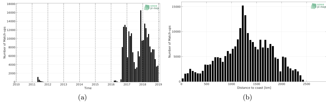
Figure 1: Number of match-ups between Surface drifters and SMOS L2 v662 (ESA) SSS as a function of time (a) and as function of the distance to coast (b) over the North Pacific Ocean Pi-MEP region and for the full satellite product period.
