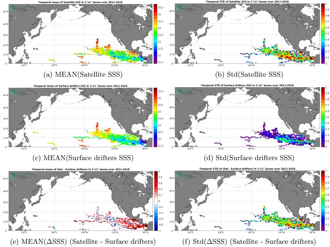
Figure 5: Temporal mean (left) and Std (right) of SSS from SMOS L2 v662 (ESA) (top), Surface drifters (middle), and of \Delta SSS (Satellite - Surface drifters). Only match-up pairs are used to generate these maps.
