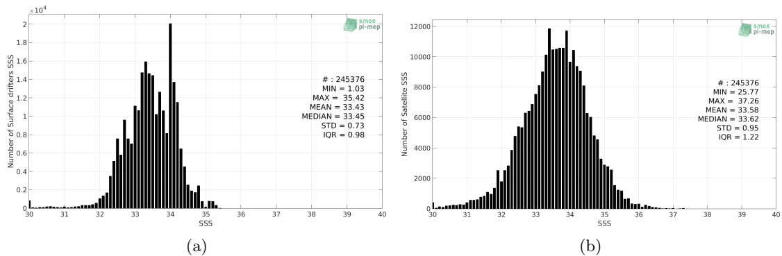
Figure 2: Histograms of SSS from Surface drifters (a) and SMOS L2 v662 (ESA) (b) considering all match-up pairs per bins of 0.1 over the North Pacific Ocean Pi-MEP region and for the full satellite product period.
