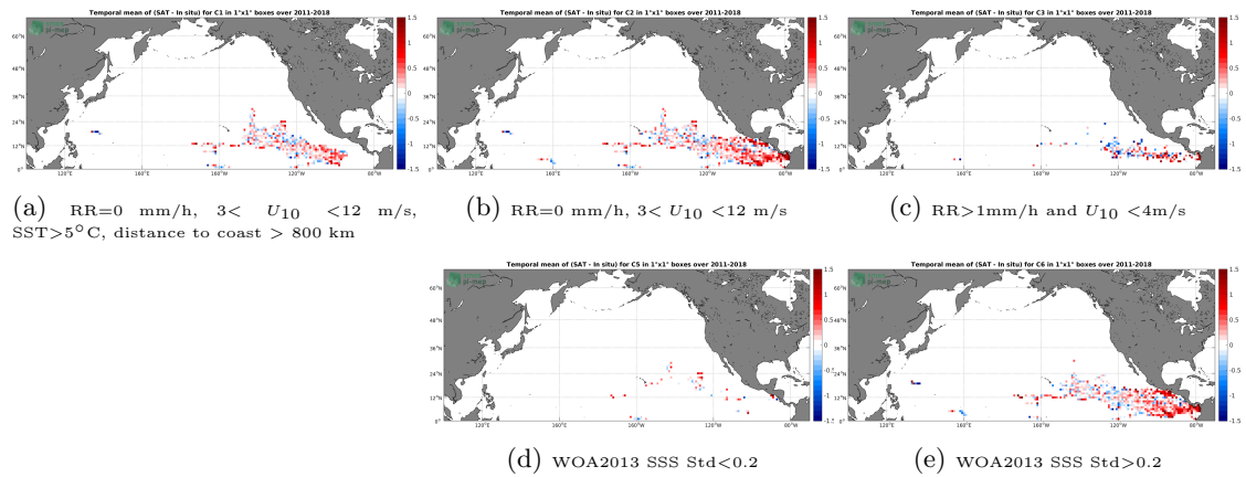
Figure 11: Temporal mean gridded over spatial boxes of size 1^\circ \times 1^\circ of \Delta SSS (SMOS L2 v662 (ESA) - Surface drifters) for 5 different subdatasets corresponding to:RR=0 mm/h, 3 < U_{10} < 12 m/s, SST >5^\circ\text{C} , distance to coast > 800 km (a), RR=0 mm/h, 3 < U_{10} < 12 m/s (b), RR >1 mm/h and U_{10} < 4 m/s (c), WOA2013 SSS Std <0.2 (d), WOA2013 SSS Std >0.2 (e).
