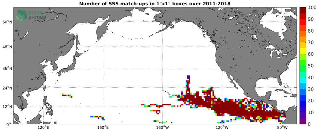
Figure 3: Number of SSS match-ups between Surface drifters SSS and the SMOS L2 v662 (ESA) SSS product for the North Pacific Ocean Pi-MEP region over 1^\circ \times 1^\circ boxes and for the full satellite product period.
