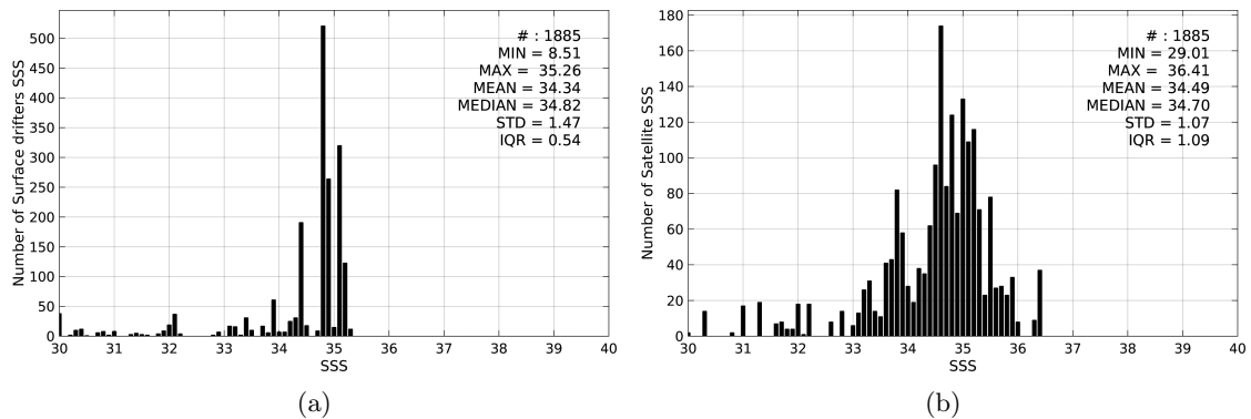
Figure 2: Histograms of SSS from Surface drifters (a) and SMOS-L2-DPGS-v662 (b) considering all match-up pairs per bins of 0.1 over the North Pacific Ocean Pi-MEP region and for the full satellite product period.
