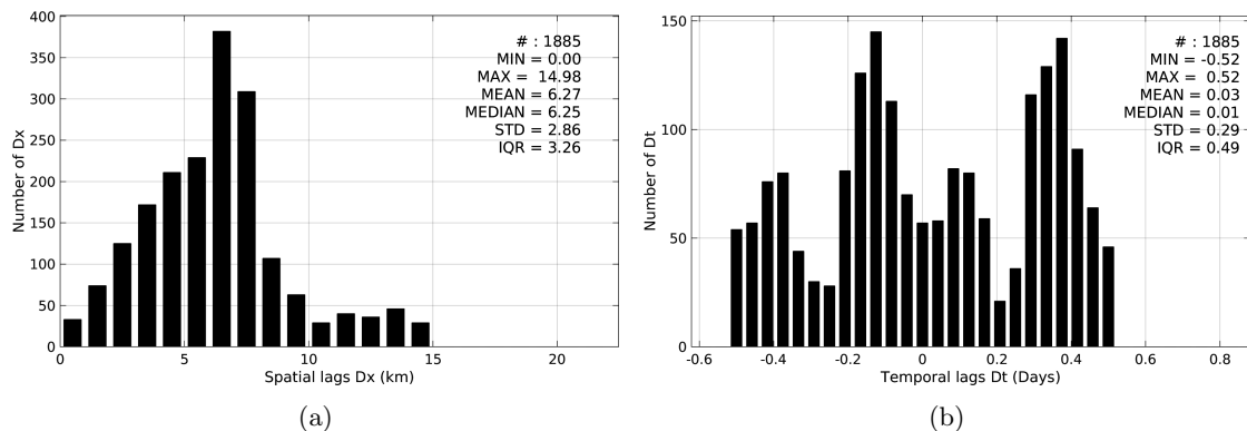
Figure 4: Histograms of the spatial (a) and temporal (b) lags between the time of the Surface drifters measurements and the date of the corresponding SMOS-L2-DPGS-v662 SSS product.
