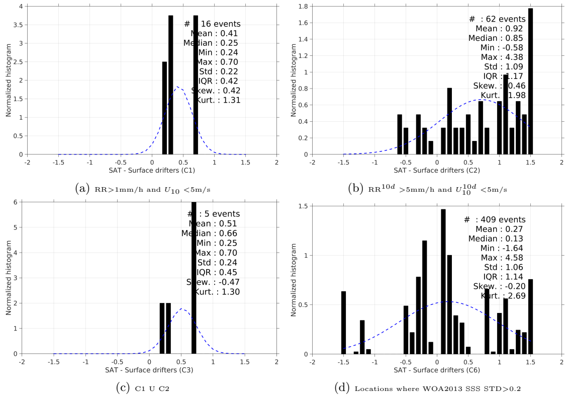
Figure 12: Normalized histogram of \Delta\text{SSS} (SMOS-L2-DPGS-v662 - Surface drifters) for 6 different subdatasets corresponding to: RR > 1mm/h and U_{10} < 5\text{m/s} (a), RR^{10d} > 5\text{mm/h} and U_{10}^{10d} < 5\text{m/s} (b), C1 U C2 (c), Locations where WOA2013 SSS STD > 0.2 (d).
