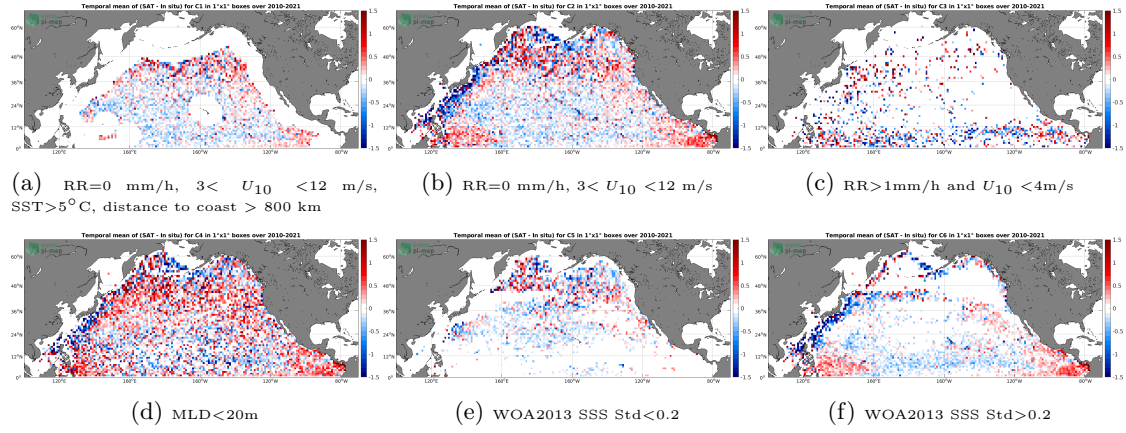
Figure 12: Temporal mean gridded over spatial boxes of size 1^\circ \times 1^\circ of \Delta SSS (SMOS SSS L2 v662 (ESA) - Argo) for 6 different subdatasets corresponding to: RR=0 mm/h, 3 < U_{10} < 12 m/s, SST > 5^\circ C , distance to coast > 800 km (a), RR=0 mm/h, 3 < U_{10} < 12 m/s (b), RR > 1 mm/h and U_{10} < 4 m/s (c), MLD < 20 m (d), WOA2013 SSS Std < 0.2 (e), WOA2013 SSS Std > 0.2 (f).
