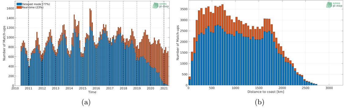
Figure 1: Number of match-ups between Argo and SMOS SSS L2 v662 (ESA) SSS as a function of time (a) and as function of the distance to coast (b) over the North Pacific Ocean Pi-MEP region and for the full satellite product period.
