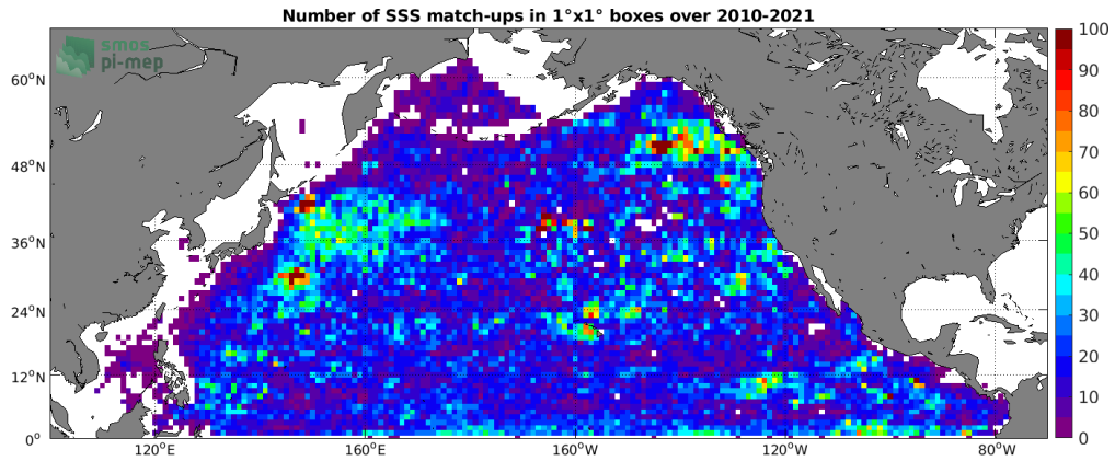
Figure 4: Number of SSS match-ups between Argo SSS and the SMOS SSS L2 v662 (ESA) SSS product for the North Pacific Ocean Pi-MEP region over 1^\circ \times 1^\circ boxes and for the full satellite product period.
