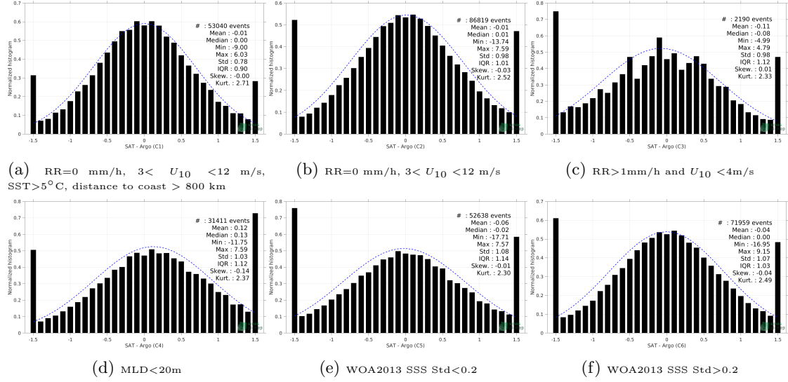
Figure 13: Normalized histogram of \Delta\text{SSS} (SMOS SSS L2 v662 (ESA) - Argo) for 6 different subdatasets corresponding to: RR=0 mm/h, 3 < U_{10} < 12 m/s, SST>5°C, distance to coast > 800 km (a), RR=0 mm/h, 3 < U_{10} < 12 m/s (b), RR>1mm/h and U_{10} < 4 m/s (c), MLD<20m (d), WOA2013 SSS Std<0.2 (e), WOA2013 SSS Std>0.2 (f).
