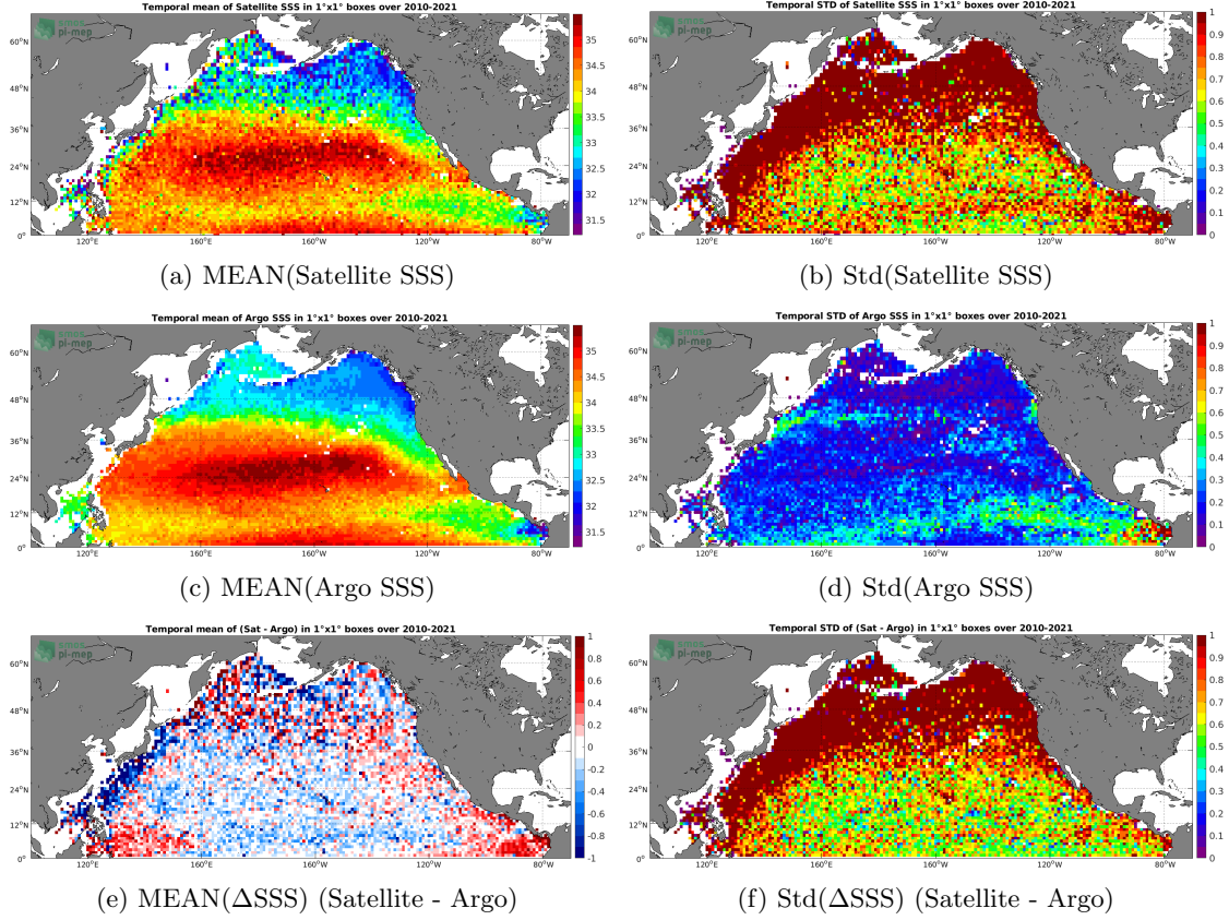
Figure 6: Temporal mean (left) and Std (right) of SSS from SMOS SSS L2 v662 (ESA) (top), Argo (middle), and of \Delta SSS (Satellite - Argo). Only match-up pairs are used to generate these maps.
