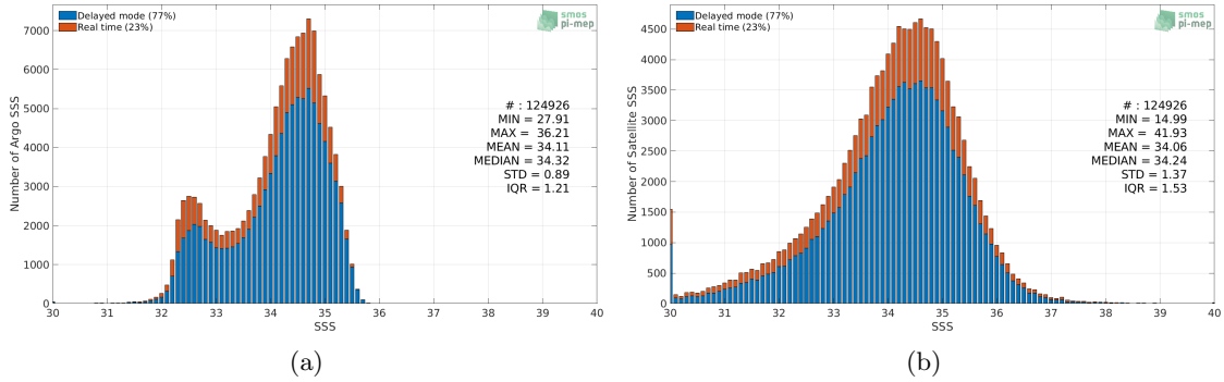
Figure 2: Histograms of SSS from Argo (a) and SMOS SSS L2 v662 (ESA) (b) considering all match-up pairs per bins of 0.1 over the North Pacific Ocean Pi-MEP region and for the full satellite product period.
