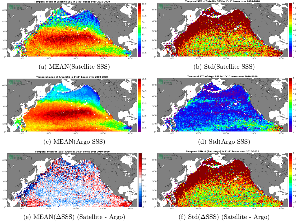
Figure 6: Temporal mean (left) and Std (right) of SSS from SMOS L2 v662 (ESA) (top), Argo (middle), and of \Delta SSS (Satellite - Argo). Only match-up pairs are used to generate these maps.
