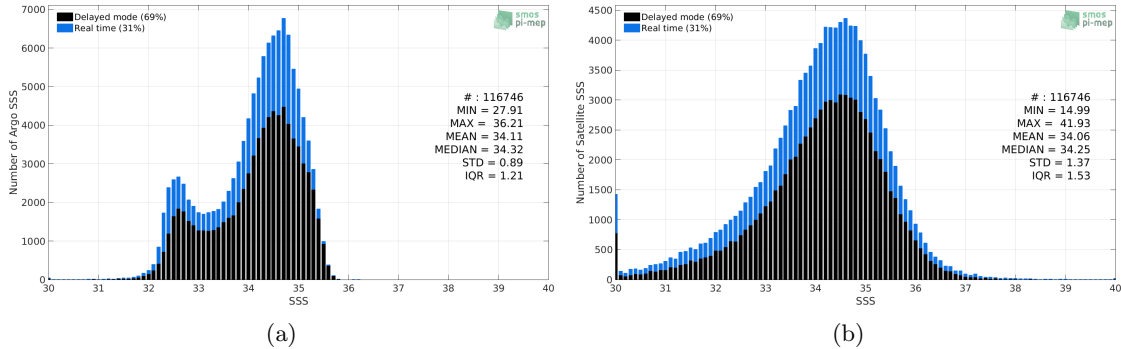
Figure 2: Histograms of SSS from Argo (a) and SMOS L2 v662 (ESA) (b) considering all match-up pairs per bins of 0.1 over the North Pacific Ocean Pi-MEP region and for the full satellite product period.
