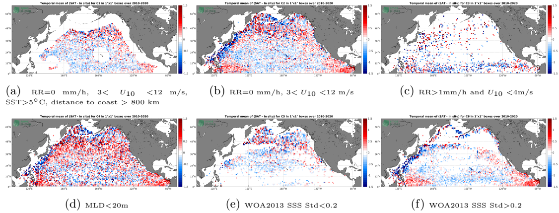
Figure 12: Temporal mean gridded over spatial boxes of size 1^\circ \times 1^\circ of \Delta SSS (SMOS L2 v662 (ESA) - Argo) for 6 different subdatasets corresponding to: RR=0 mm/h, 3 < U_{10} < 12 m/s, SST > 5^\circ\text{C} , distance to coast > 800 km (a), RR=0 mm/h, 3 < U_{10} < 12 m/s (b), RR > 1 mm/h and U_{10} < 4 m/s (c), MLD < 20 m (d), WOA2013 SSS Std < 0.2 (e), WOA2013 SSS Std > 0.2 (f).
