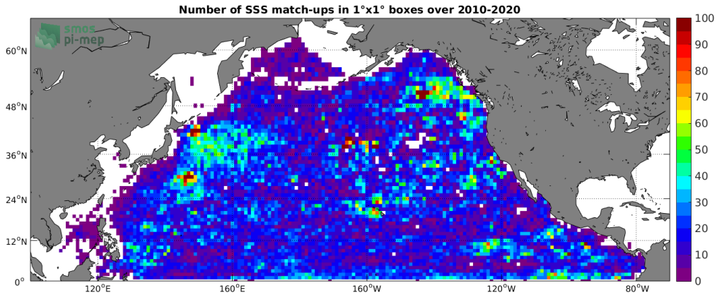
Figure 4: Number of SSS match-ups between Argo SSS and the SMOS L2 v662 (ESA) SSS product for the North Pacific Ocean Pi-MEP region over 1^\circ \times 1^\circ boxes and for the full satellite product period.
