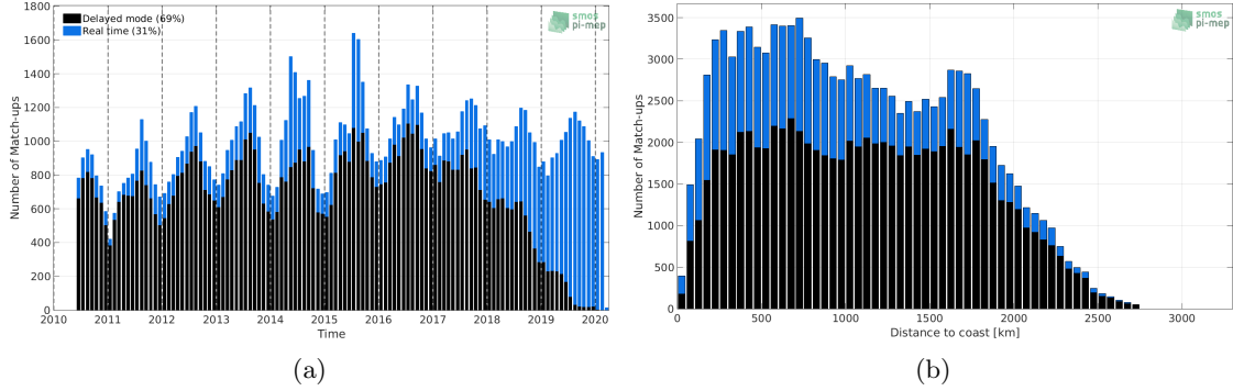
Figure 1: Number of match-ups between Argo and SMOS L2 v662 (ESA) SSS as a function of time (a) and as function of the distance to coast (b) over the North Pacific Ocean Pi-MEP region and for the full satellite product period.
