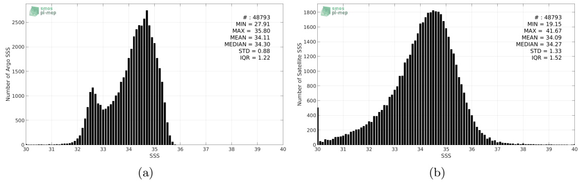
Figure 2: Histograms of SSS from Argo (a) and SMOS-L2-DPGS-v662 (b) considering all match-up pairs per bins of 0.1 over the North Pacific Ocean Pi-MEP region and for the full satellite product period.
