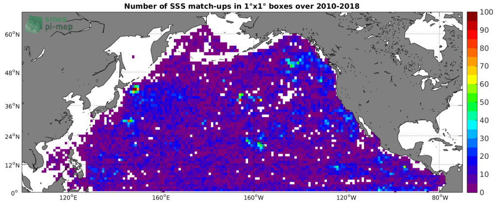
Figure 4: Number of SSS match-ups between Argo SSS and the SMOS-L2-DPGS-v662 SSS product for the North Pacific Ocean Pi-MEP region over 1^\circ \times 1^\circ boxes and for the full satellite product period.
