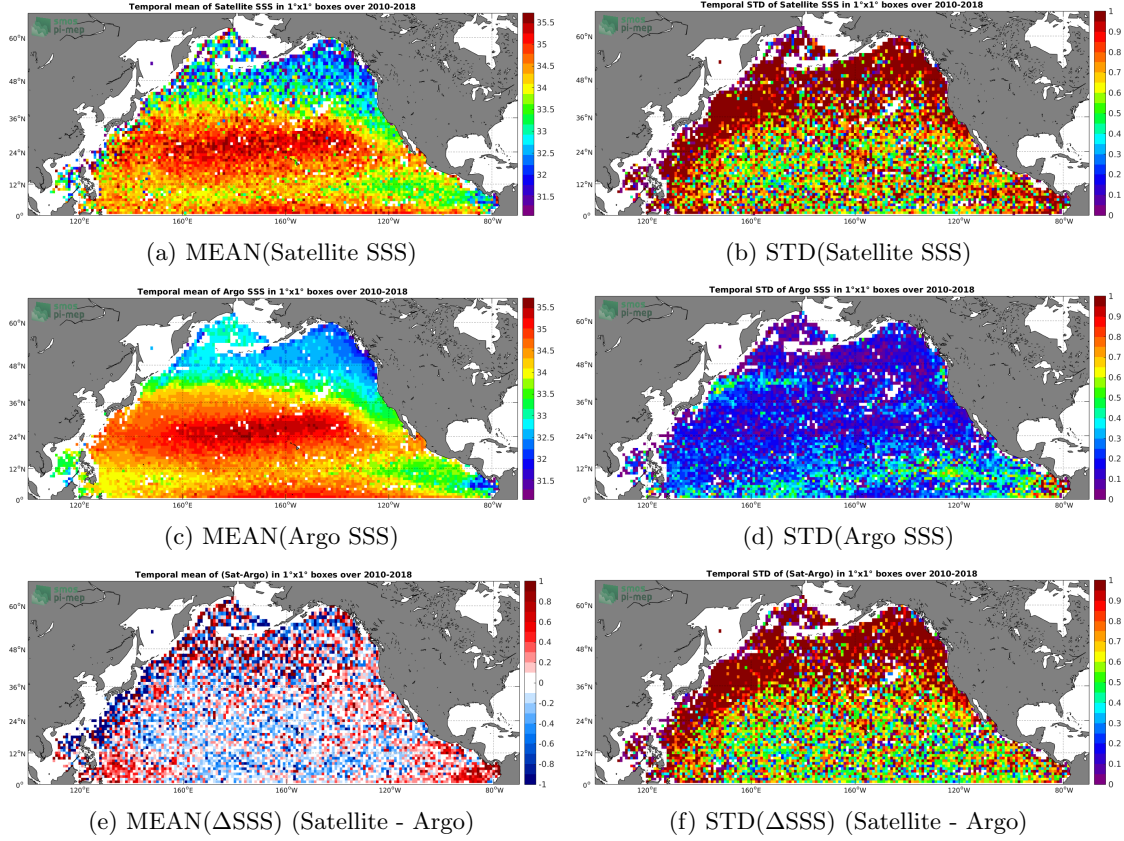
Figure 6: Temporal mean (left) and STD (right) of SSS from SMOS-L2-DPGS-v662 (top), Argo (middle), and of \Delta SSS (Satellite - Argo). Only match-up pairs are used to generate these maps.
