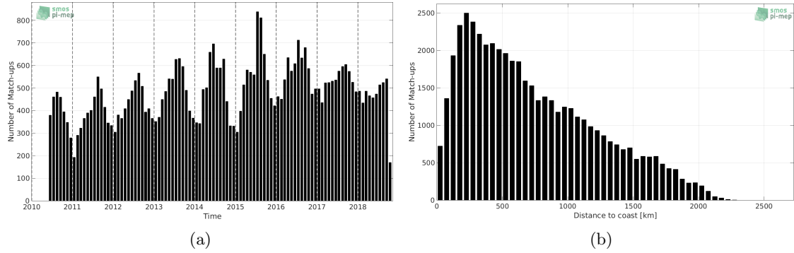
Figure 1: Number of match-ups between Argo and SMOS-L2-DPGS-v662 SSS as a function of time (a) and as function of the distance to coast (b) over the North Pacific Ocean Pi-MEP region and for the full satellite product period.
