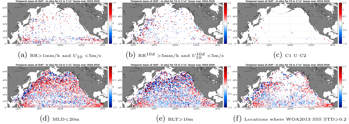
Figure 12: Temporal mean gridded over spatial boxes of size 1^\circ \times 1^\circ of \Delta\text{SSS} (SMOS-L2-DPGS-v662 - Argo) for 6 different subdatasets corresponding to: \text{RR} > 1\text{mm/h} and U_{10} < 5\text{m/s} (a), \text{RR}^{10d} > 5\text{mm/h} and U_{10}^{10d} < 5\text{m/s} (b), C1 U C2 (c), \text{MLD} < 20\text{m} (d), \text{BLT} > 10\text{m} (e), Locations where WOA2013 SSS STD > 0.2 (f).
