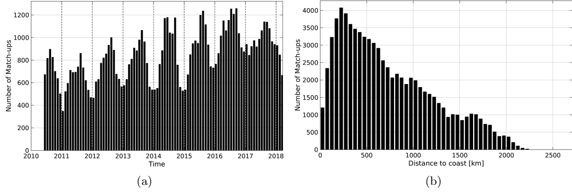
Figure 1: Number of match-ups between Argo and SMOS-L2-DPGS-v662 SSS as a function of time (a) and as function of the distance to coast (b) over the North Pacific Ocean Pi-MEP region and for the full satellite product period.
