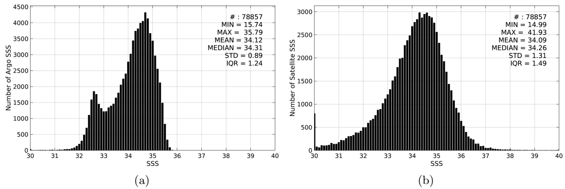
Figure 2: Histograms of SSS from Argo (a) and SMOS-L2-DPGS-v662 (b) considering all match-up pairs per bins of 0.1 over the North Pacific Ocean Pi-MEP region and for the full satellite product period.
