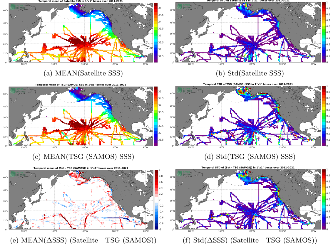
Figure 6: Temporal mean (left) and Std (right) of SSS from SMAP SSS L4 OI v1 - 7 Days (IPRC) (top), TSG (SAMOS) (middle), and of \Delta\text{SSS} (Satellite - TSG (SAMOS)). Only match-up pairs are used to generate these maps.
