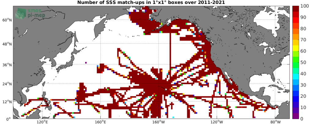
Figure 4: Number of SSS match-ups between TSG (SAMOS) SSS and the SMAP SSS L4 OI v1 - 7 Days (IPRC) SSS product for the North Pacific Ocean Pi-MEP region over 1^\circ \times 1^\circ boxes and for the full satellite product period.
