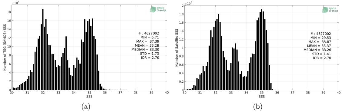
Figure 2: Histograms of SSS from TSG (SAMOS) (a) and SMAP SSS L4 OI v1 - 7 Days (IPRC) (b) considering all match-up pairs per bins of 0.1 over the North Pacific Ocean Pi-MEP region and for the full satellite product period.
