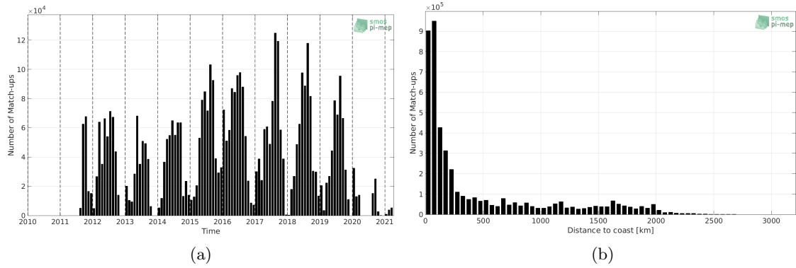
Figure 1: Number of match-ups between TSG (SAMOS) and SMAP SSS L4 OI v1 - 7 Days (IPRC) SSS as a function of time (a) and as function of the distance to coast (b) over the North Pacific Ocean Pi-MEP region and for the full satellite product period.
