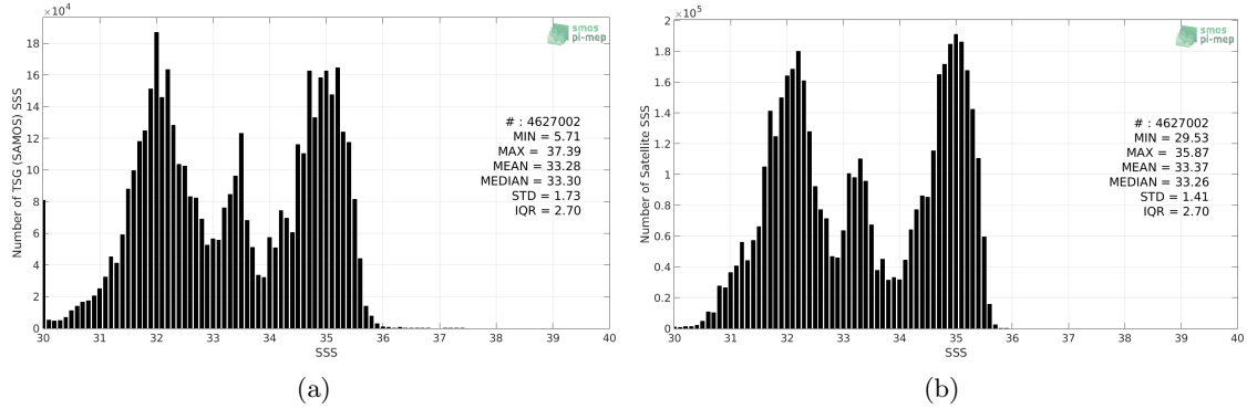
Figure 2: Histograms of SSS from TSG (SAMOS) (a) and SMAP SSS L4 OI v1 - 7day (IPRC) (b) considering all match-up pairs per bins of 0.1 over the North Pacific Ocean Pi-MEP region and for the full satellite product period.
