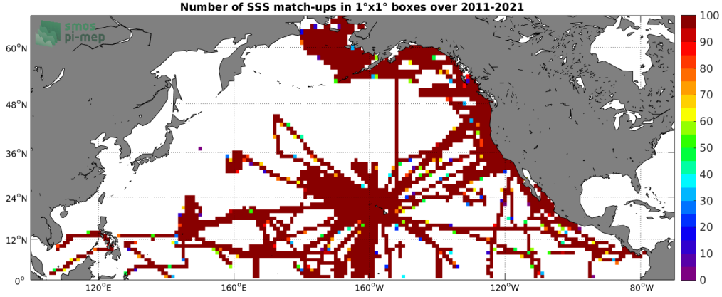
Figure 4: Number of SSS match-ups between TSG (SAMOS) SSS and the SMAP SSS L4 OI v1 - 7day (IPRC) SSS product for the North Pacific Ocean Pi-MEP region over 1^\circ \times 1^\circ boxes and for the full satellite product period.
