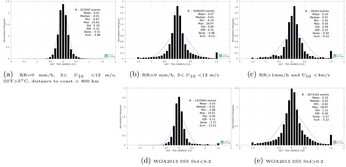
Figure 13: Normalized histogram of \Delta SSS (SMAP SSS L4 OI v1 - 7day (IPRC) - TSG (SAMOS)) for 5 different subdatasets corresponding to: RR=0 mm/h, 3 < U_{10} < 12 m/s, SST>5°C, distance to coast > 800 km (a), RR=0 mm/h, 3 < U_{10} < 12 m/s (b), RR>1mm/h and U_{10} < 4 m/s (c), WOA2013 SSS Std<0.2 (d), WOA2013 SSS Std>0.2 (e).
