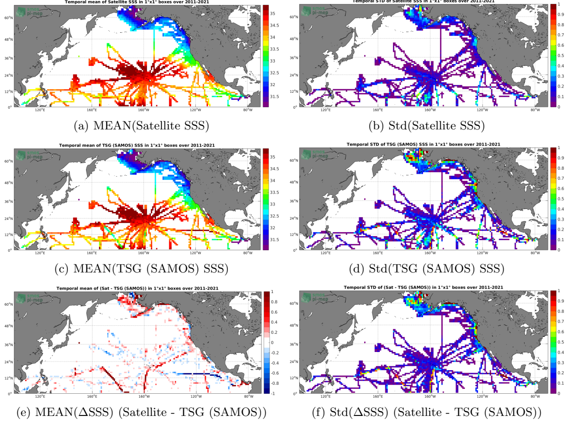
Figure 6: Temporal mean (left) and Std (right) of SSS from SMAP SSS L4 OI v1 - 7day (IPRC) (top), TSG (SAMOS) (middle), and of \Delta\text{SSS} (Satellite - TSG (SAMOS)). Only match-up pairs are used to generate these maps.
