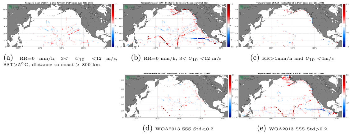
Figure 12: Temporal mean gridded over spatial boxes of size 1^\circ \times 1^\circ of \Delta SSS (SMAP SSS L4 OI v1 - 7day (IPRC) - TSG (SAMOS)) for 5 different subdatasets corresponding to: RR=0 mm/h, 3 < U_{10} < 12 m/s, SST>5°C, distance to coast > 800 km (a), RR=0 mm/h, 3 < U_{10} < 12 m/s (b), RR>1mm/h and U_{10} < 4 m/s (c), WOA2013 SSS Std<0.2 (d), WOA2013 SSS Std>0.2 (e).
