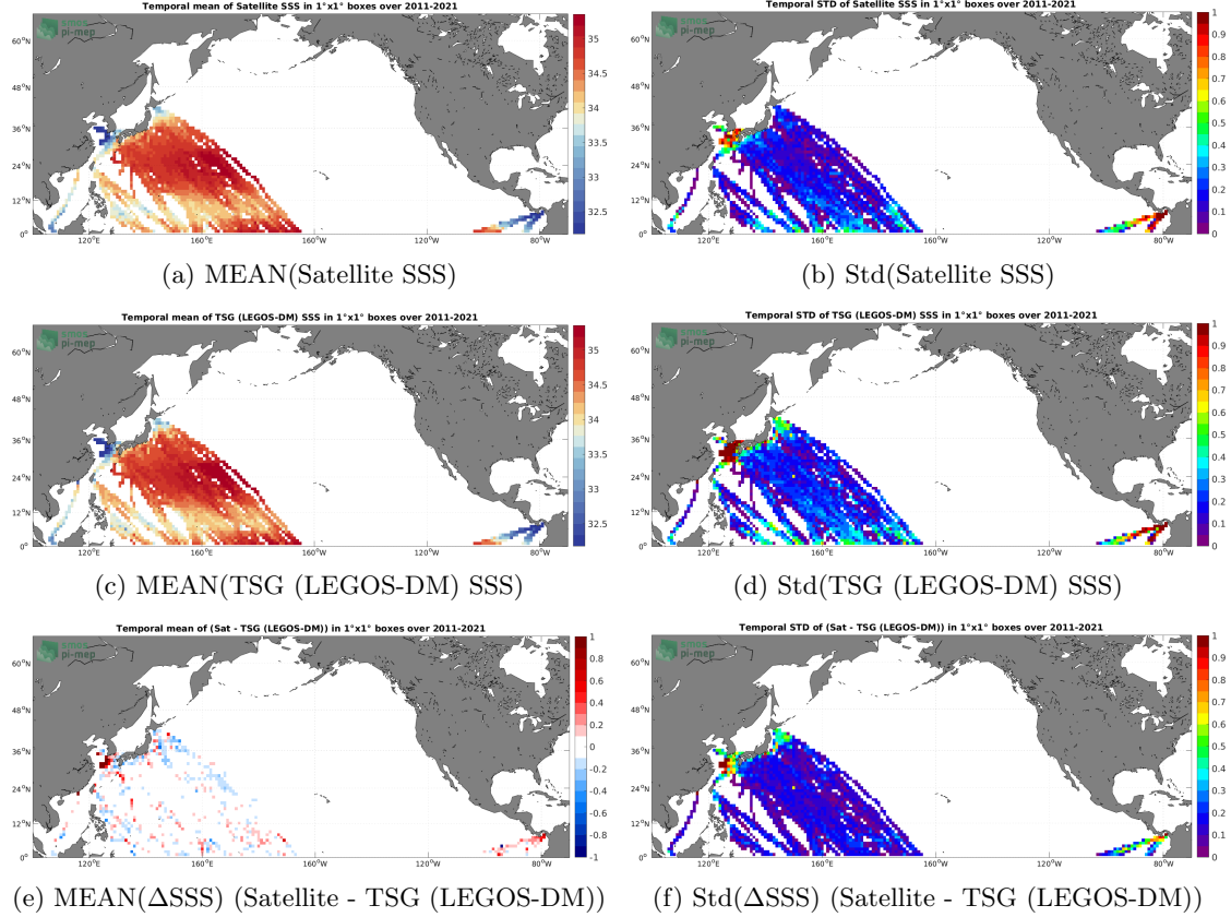
Figure 6: Temporal mean (left) and Std (right) of SSS from SMAP SSS L4 OI v1 - 7 Days (IPRC) (top), TSG (LEGOS-DM) (middle), and of \Delta\text{SSS} (Satellite - TSG (LEGOS-DM)). Only match-up pairs are used to generate these maps.
