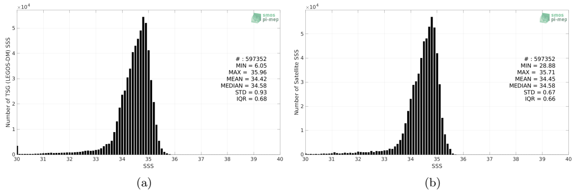
Figure 2: Histograms of SSS from TSG (LEGOS-DM) (a) and SMAP SSS L4 OI v1 - 7 Days (IPRC) (b) considering all match-up pairs per bins of 0.1 over the North Pacific Ocean Pi-MEP region and for the full satellite product period.
