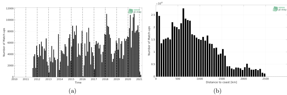
Figure 1: Number of match-ups between TSG (LEGOS-DM) and SMAP SSS L4 OI v1 - 7 Days (IPRC) SSS as a function of time (a) and as function of the distance to coast (b) over the North Pacific Ocean Pi-MEP region and for the full satellite product period.
