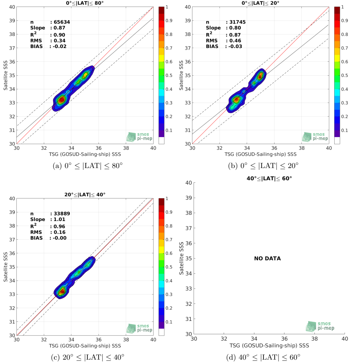
Figure 9: Contour maps of the concentration of SMAP SSS L4 OI v1 - 7day (IPRC) SSS (y-axis) versus TSG (GOSUD-Sailing-ship) SSS (x-axis) at match-up pairs for different latitude bands. For each plot, the red line shows x=y . The black thin and dashed lines indicate a linear fit through the data cloud and the \pm 95\% confidence levels, respectively. The number match-up pairs n , the slope and R^2 coefficient of the linear fit, the root mean square (RMS) and the mean bias between satellite and in situ data are indicated for each latitude band in each plots.
