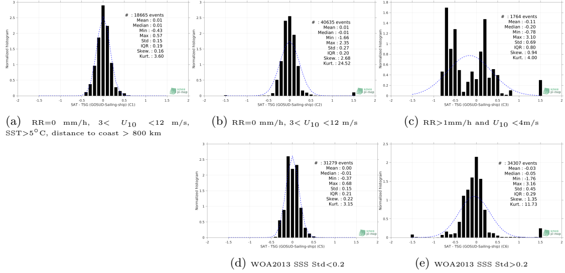
Figure 13: Normalized histogram of \Delta SSS (SMAP SSS L4 OI v1 - 7day (IPRC) - TSG (GOSUD-Sailing-ship)) for 5 different subdatasets corresponding to: RR=0 mm/h, 3 < U_{10} < 12 m/s, SST>5°C, distance to coast > 800 km (a), RR=0 mm/h, 3 < U_{10} < 12 m/s (b), RR>1mm/h and U_{10} < 4 m/s (c), WOA2013 SSS Std<0.2 (d), WOA2013 SSS Std>0.2 (e).
