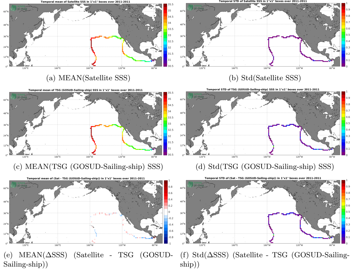
Figure 6: Temporal mean (left) and Std (right) of SSS from SMAP SSS L4 OI v1 - 7day (IPRC) (top), TSG (GOSUD-Sailing-ship) (middle), and of \Delta\text{SSS} (Satellite - TSG (GOSUD-Sailing-ship)). Only match-up pairs are used to generate these maps.
