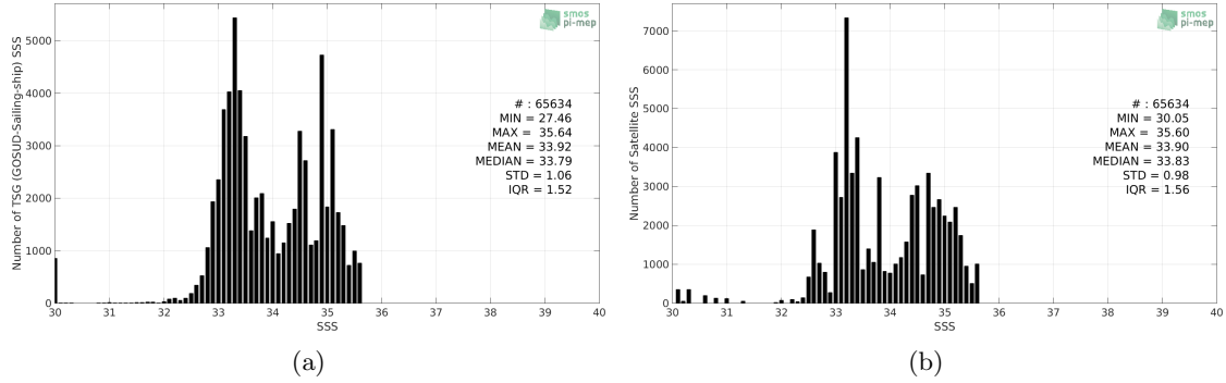
Figure 2: Histograms of SSS from TSG (GOSUD-Sailing-ship) (a) and SMAP SSS L4 OI v1 - 7day (IPRC) (b) considering all match-up pairs per bins of 0.1 over the North Pacific Ocean Pi-MEP region and for the full satellite product period.
