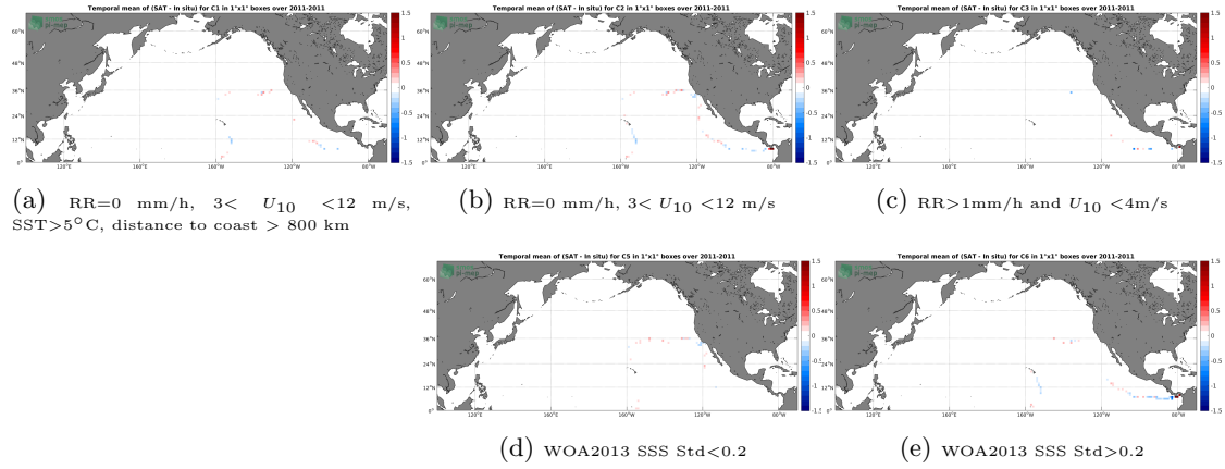
Figure 12: Temporal mean gridded over spatial boxes of size 1^\circ \times 1^\circ of \Delta SSS (SMAP SSS L4 OI v1 - 7day (IPRC) - TSG (GOSUD-Sailing-ship)) for 5 different subdatasets corresponding to: RR=0 mm/h, 3 < U_{10} < 12 m/s, SST >5^\circ\text{C} , distance to coast > 800 km (a), RR=0 mm/h, 3 < U_{10} < 12 m/s (b), RR >1 mm/h and U_{10} < 4 m/s (c), WOA2013 SSS Std <0.2 (d), WOA2013 SSS Std >0.2 (e).
