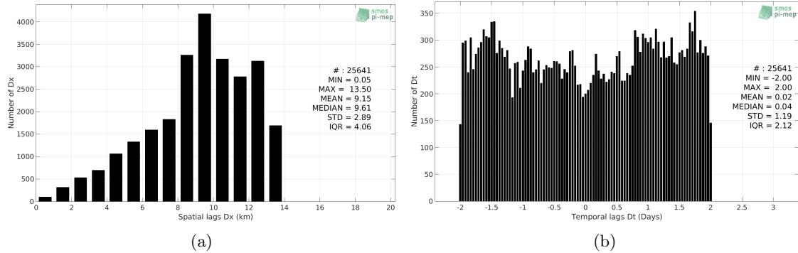
Figure 5: Histograms of the spatial (a) and temporal (b) lags between the location/time of the TSG (GOSUD-Research-vessel) measurement and the date of the corresponding SMAP SSS L4 OI v1 - 7day (IPRC) SSS pixel.
