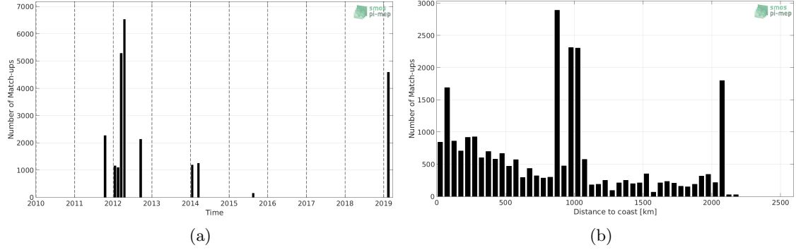
Figure 1: Number of match-ups between TSG (GOSUD-Research-vessel) and SMAP SSS L4 OI v1 - 7day (IPRC) SSS as a function of time (a) and as function of the distance to coast (b) over the North Pacific Ocean Pi-MEP region and for the full satellite product period.
