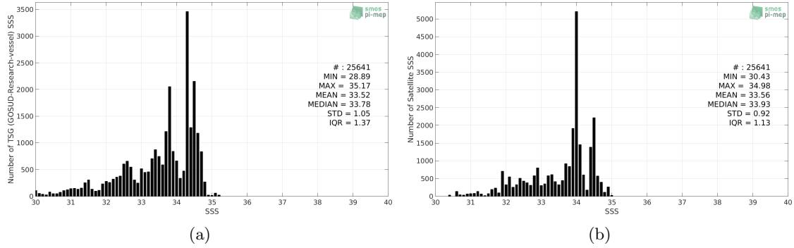
Figure 2: Histograms of SSS from TSG (GOSUD-Research-vessel) (a) and SMAP SSS L4 OI v1 - 7day (IPRC) (b) considering all match-up pairs per bins of 0.1 over the North Pacific Ocean Pi-MEP region and for the full satellite product period.
