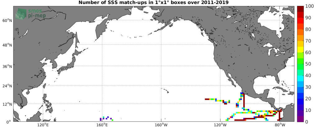
Figure 4: Number of SSS match-ups between TSG (GOSUD-Research-vessel) SSS and the SMAP SSS L4 OI v1 - 7day (IPRC) SSS product for the North Pacific Ocean Pi-MEP region over 1^\circ \times 1^\circ boxes and for the full satellite product period.
