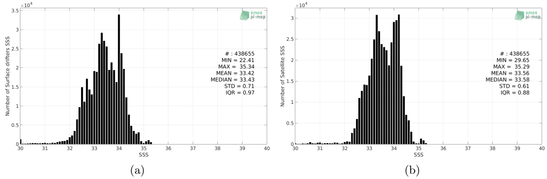
Figure 2: Histograms of SSS from Surface drifters (a) and SMAP SSS L4 OI v1 - 7 Days (IPRC) (b) considering all match-up pairs per bins of 0.1 over the North Pacific Ocean Pi-MEP region and for the full satellite product period.
