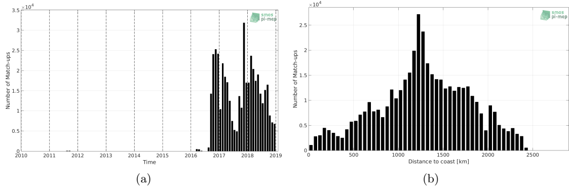
Figure 1: Number of match-ups between Surface drifters and SMAP SSS L4 OI v1 - 7 Days (IPRC) SSS as a function of time (a) and as function of the distance to coast (b) over the North Pacific Ocean Pi-MEP region and for the full satellite product period.
