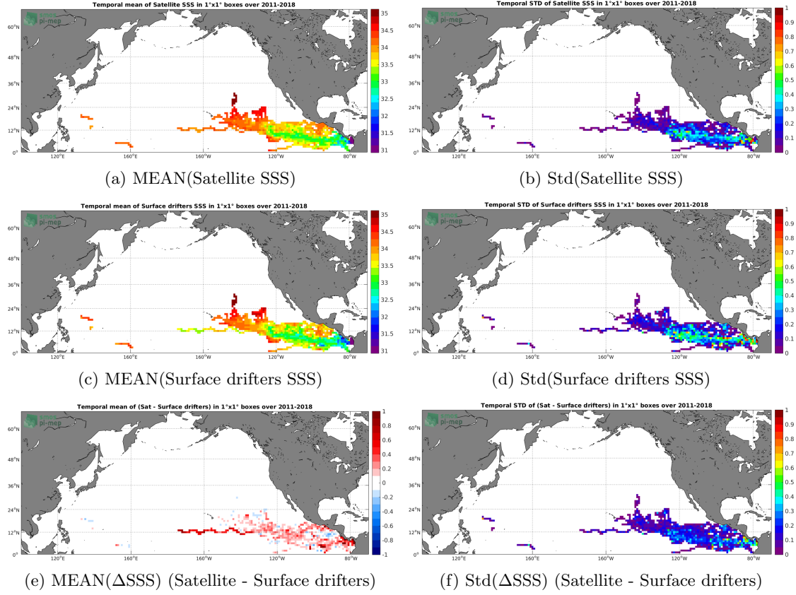
Figure 5: Temporal mean (left) and Std (right) of SSS from SMAP SSS L4 OI v1 - 7 Days (IPRC) (top), Surface drifters (middle), and of \Delta SSS (Satellite - Surface drifters). Only match-up pairs are used to generate these maps.
