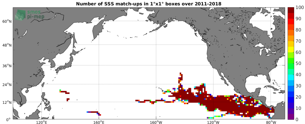
Figure 3: Number of SSS match-ups between Surface drifters SSS and the SMAP SSS L4 OI v1 - 7 Days (IPRC) SSS product for the North Pacific Ocean Pi-MEP region over 1^\circ \times 1^\circ boxes and for the full satellite product period.
