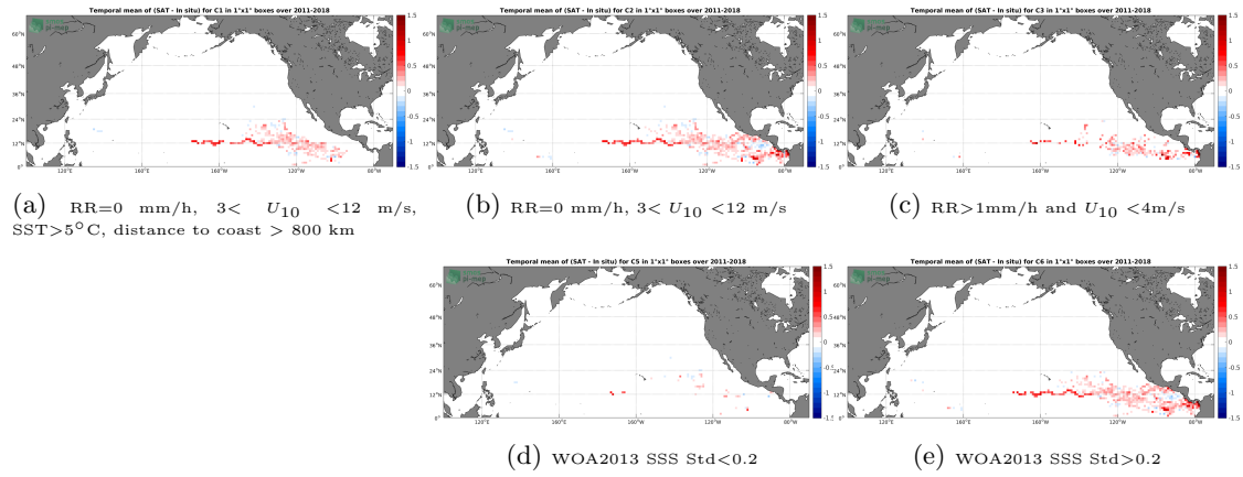
Figure 11: Temporal mean gridded over spatial boxes of size 1^\circ \times 1^\circ of \Delta SSS (SMAP SSS L4 OI v1 - 7 Days (IPRC) - Surface drifters) for 5 different subdatasets corresponding to:RR=0 mm/h, 3 < U_{10} < 12 m/s, SST >5^\circ\text{C} , distance to coast > 800 km (a), RR=0 mm/h, 3 < U_{10} < 12 m/s (b), RR >1 mm/h and U_{10} < 4 m/s (c), WOA2013 SSS Std <0.2 (d), WOA2013 SSS Std >0.2 (e).
