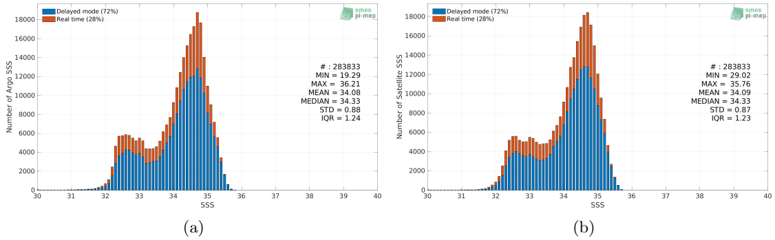
Figure 2: Histograms of SSS from Argo (a) and SMAP SSS L4 OI v1 - 7 Days (IPRC) (b) considering all match-up pairs per bins of 0.1 over the North Pacific Ocean Pi-MEP region and for the full satellite product period.
