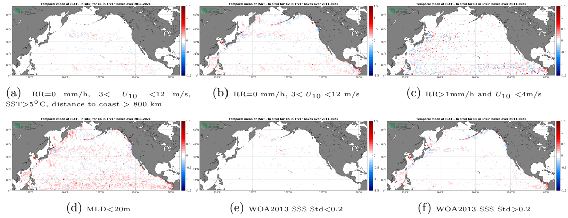
Figure 12: Temporal mean gridded over spatial boxes of size 1^\circ \times 1^\circ of \Delta SSS (SMAP SSS L4 OI v1 - 7 Days (IPRC) - Argo) for 6 different subdatasets corresponding to: RR=0 mm/h, 3 < U_{10} < 12 m/s, SST > 5^\circ C , distance to coast > 800 km (a), RR=0 mm/h, 3 < U_{10} < 12 m/s (b), RR > 1 mm/h and U_{10} < 4 m/s (c), MLD < 20 m (d), WOA2013 SSS Std < 0.2 (e), WOA2013 SSS Std > 0.2 (f).
