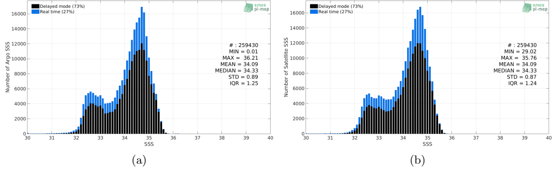
Figure 2: Histograms of SSS from Argo (a) and SMAP SSS L4 OI v1 - 7 Days (IPRC) (b) considering all match-up pairs per bins of 0.1 over the North Pacific Ocean Pi-MEP region and for the full satellite product period.
