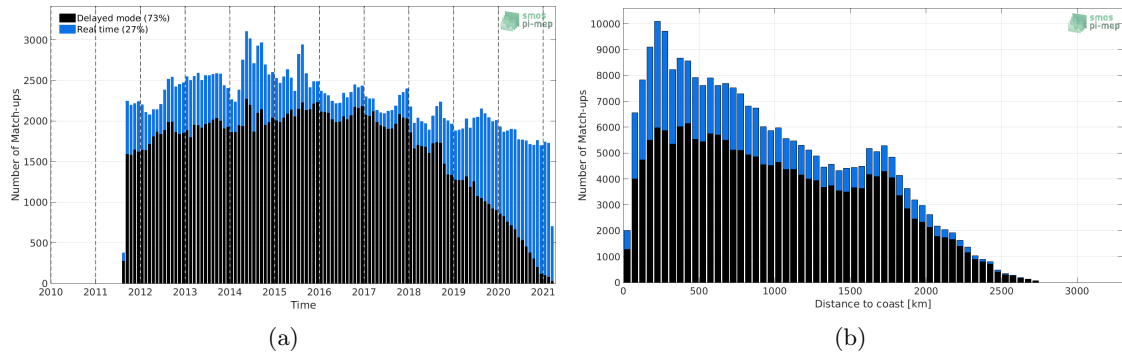
Figure 1: Number of match-ups between Argo and SMAP SSS L4 OI v1 - 7 Days (IPRC) SSS as a function of time (a) and as function of the distance to coast (b) over the North Pacific Ocean Pi-MEP region and for the full satellite product period.
