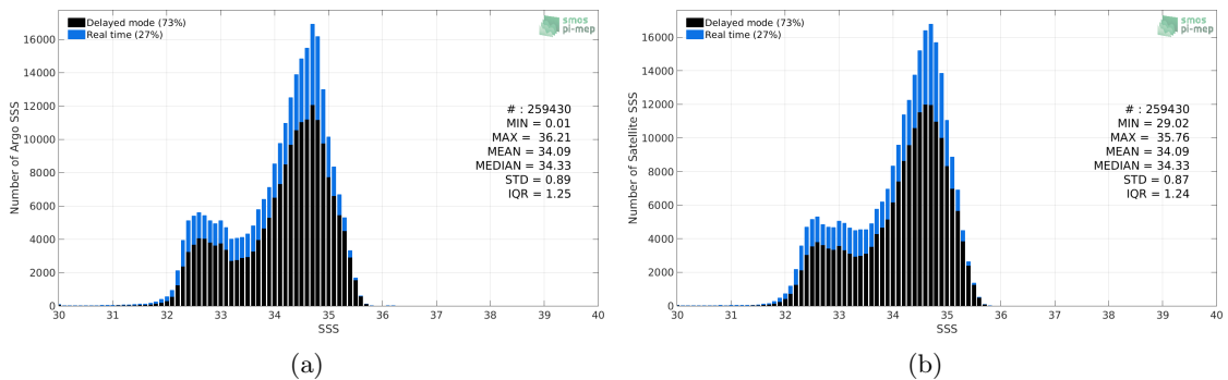
Figure 2: Histograms of SSS from Argo (a) and SMAP SSS L4 OI v1 - 7day (IPRC) (b) considering all match-up pairs per bins of 0.1 over the North Pacific Ocean Pi-MEP region and for the full satellite product period.
