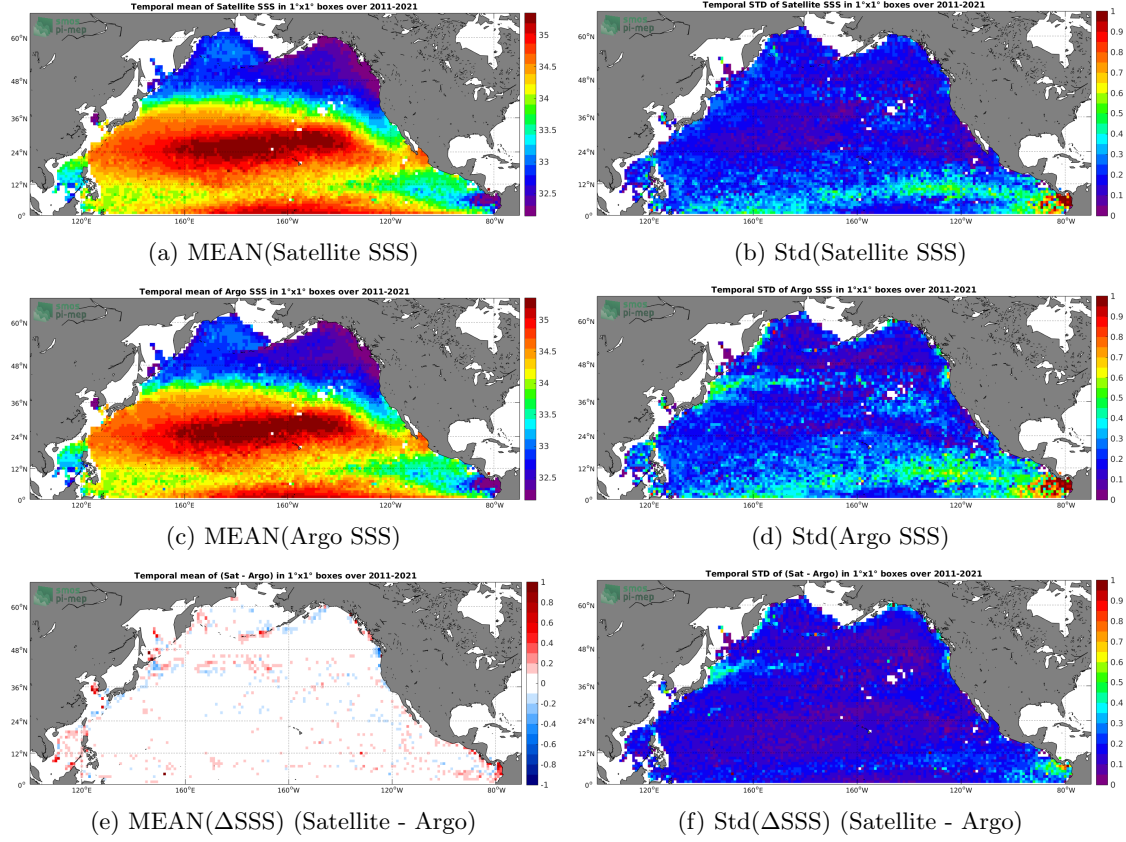
Figure 6: Temporal mean (left) and Std (right) of SSS from SMAP SSS L4 OI v1 - 7day (IPRC) (top), Argo (middle), and of \Delta SSS (Satellite - Argo). Only match-up pairs are used to generate these maps.
