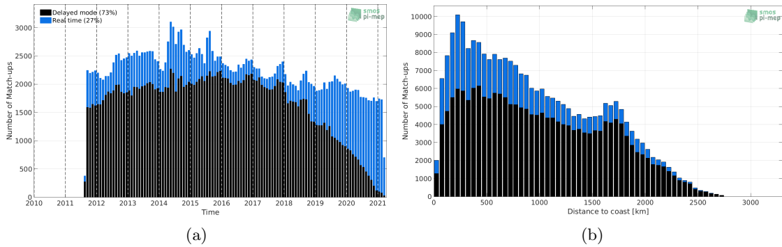
Figure 1: Number of match-ups between Argo and SMAP SSS L4 OI v1 - 7day (IPRC) SSS as a function of time (a) and as function of the distance to coast (b) over the North Pacific Ocean Pi-MEP region and for the full satellite product period.
