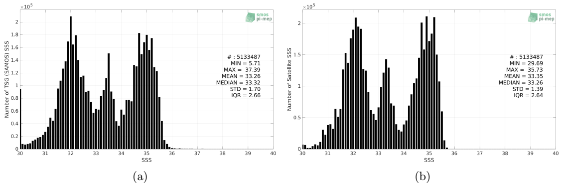
Figure 2: Histograms of SSS from TSG (SAMOS) (a) and SMAP SSS L4 OI v1 - Monthly (IPRC) (b) considering all match-up pairs per bins of 0.1 over the North Pacific Ocean Pi-MEP region and for the full satellite product period.
