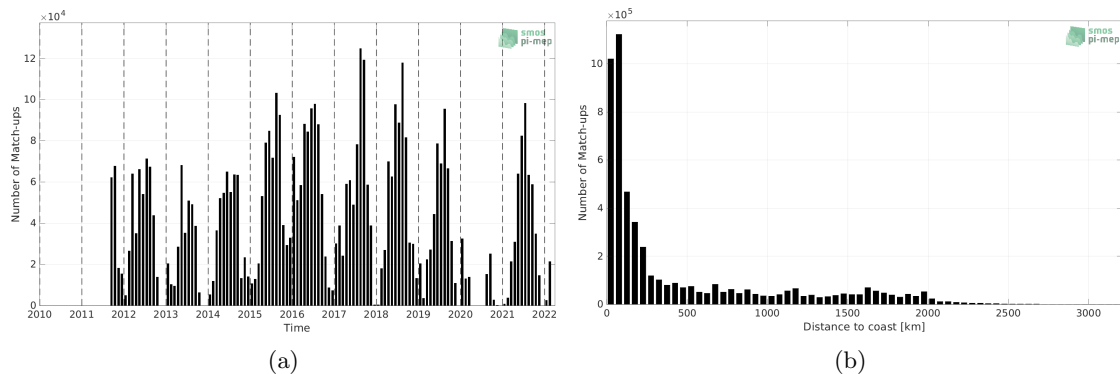
Figure 1: Number of match-ups between TSG (SAMOS) and SMAP SSS L4 OI v1 - Monthly (IPRC) SSS as a function of time (a) and as function of the distance to coast (b) over the North Pacific Ocean Pi-MEP region and for the full satellite product period.
