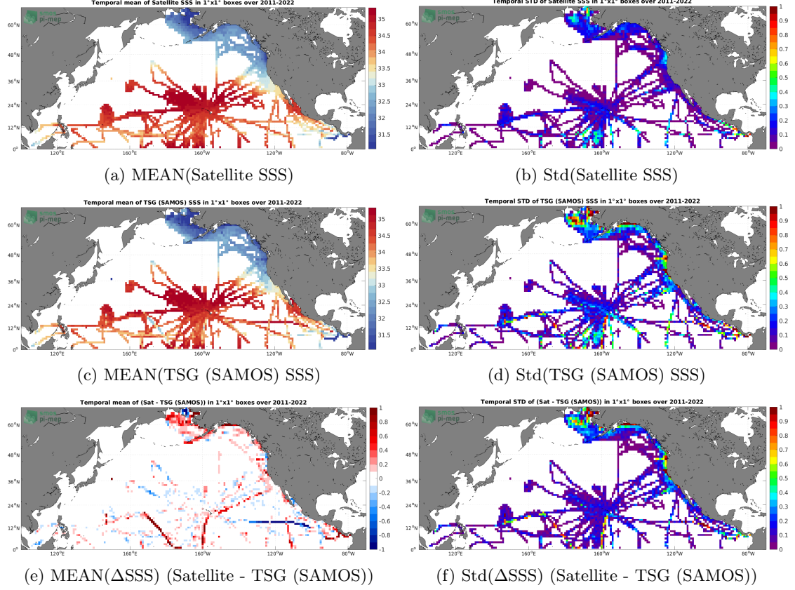
Figure 6: Temporal mean (left) and Std (right) of SSS from SMAP SSS L4 OI v1 - Monthly (IPRC) (top), TSG (SAMOS) (middle), and of \Delta\text{SSS} (Satellite - TSG (SAMOS)). Only match-up pairs are used to generate these maps.
