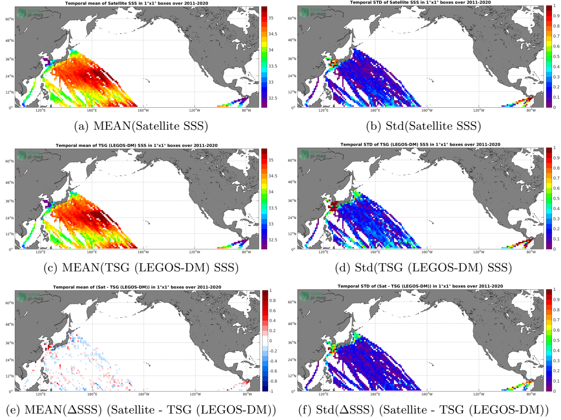
Figure 6: Temporal mean (left) and Std (right) of SSS from SMAP SSS L4 OI v1 - Monthly (IPRC) (top), TSG (LEGOS-DM) (middle), and of \Delta SSS (Satellite - TSG (LEGOS-DM)). Only match-up pairs are used to generate these maps.
