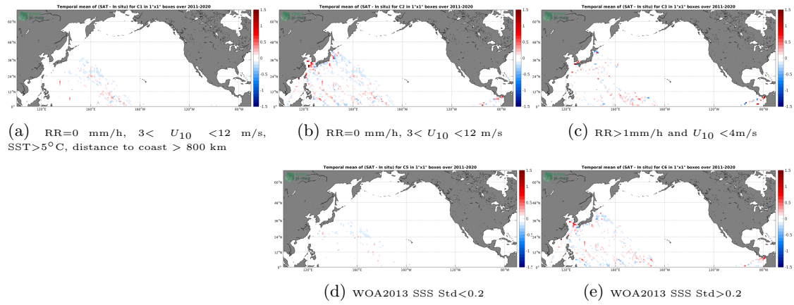
Figure 12: Temporal mean gridded over spatial boxes of size 1^\circ \times 1^\circ of \Delta SSS (SMAP SSS L4 OI v1 - Monthly (IPRC) - TSG (LEGOS-DM)) for 5 different subdatasets corresponding to: RR=0 mm/h, 3 < U_{10} < 12 m/s, SST > 5^\circ C , distance to coast > 800 km (a), RR=0 mm/h, 3 < U_{10} < 12 m/s (b), RR > 1 mm/h and U_{10} < 4 m/s (c), WOA2013 SSS Std < 0.2 (d), WOA2013 SSS Std > 0.2 (e).
