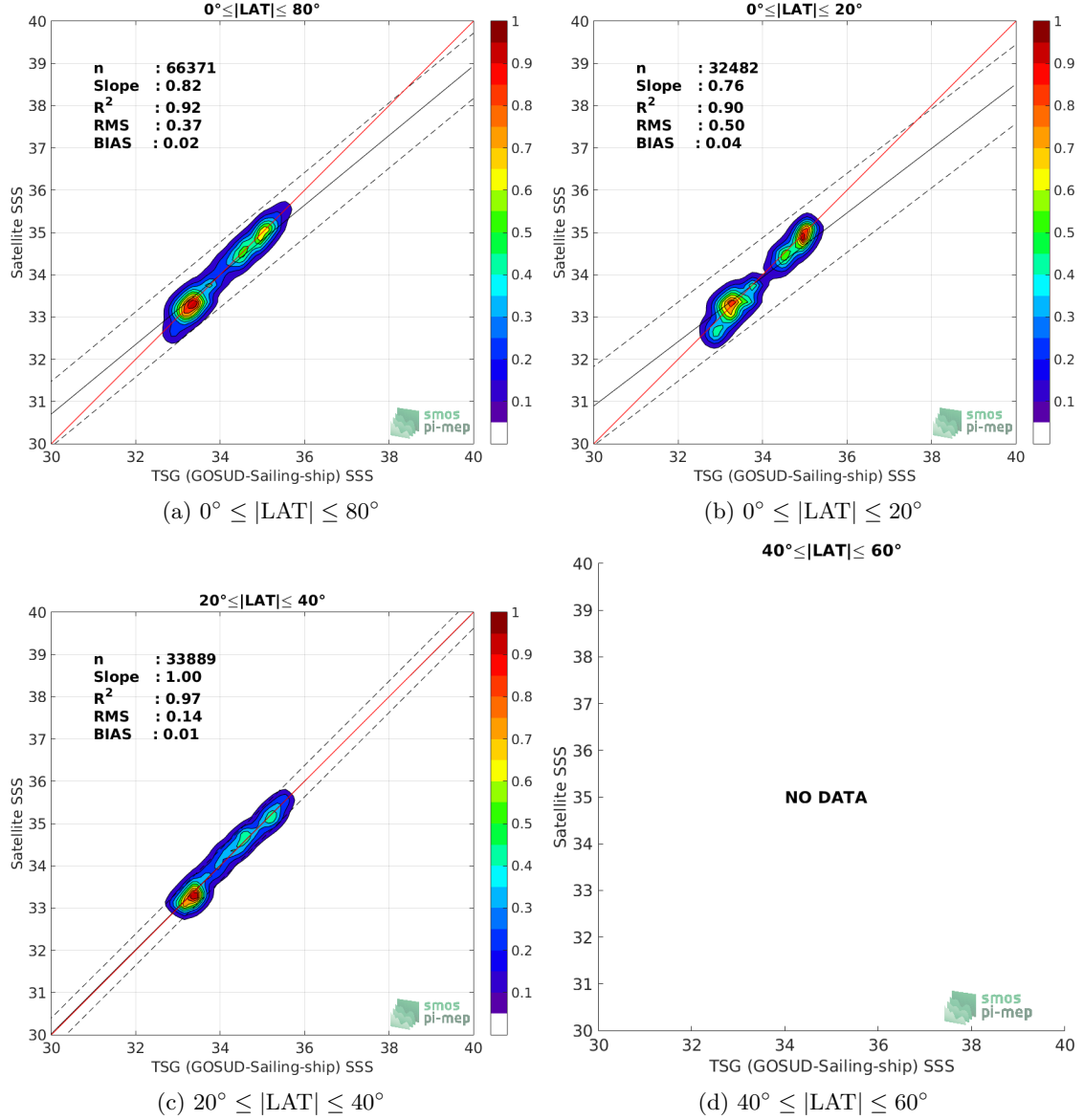
Figure 9: Contour maps of the concentration of SMAP SSS L4 OI v1 - Monthly (IPRC) SSS (y-axis) versus TSG (GOSUD-Sailing-ship) SSS (x-axis) at match-up pairs for different latitude bands. For each plot, the red line shows x=y . The black thin and dashed lines indicate a linear fit through the data cloud and the \pm 95\% confidence levels, respectively. The number match-up pairs n , the slope and R^2 coefficient of the linear fit, the root mean square (RMS) and the mean bias between satellite and in situ data are indicated for each latitude band in each plots.
