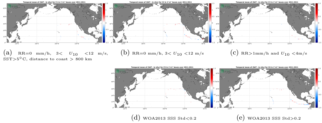
Figure 12: Temporal mean gridded over spatial boxes of size 1^\circ \times 1^\circ of \Delta SSS (SMAP SSS L4 OI v1 - Monthly (IPRC) - TSG (GOSUD-Sailing-ship)) for 5 different subdatasets corresponding to: RR=0 mm/h, 3 < U_{10} < 12 m/s, SST > 5^\circ C , distance to coast > 800 km (a), RR=0 mm/h, 3 < U_{10} < 12 m/s (b), RR > 1 mm/h and U_{10} < 4 m/s (c), WOA2013 SSS Std < 0.2 (d), WOA2013 SSS Std > 0.2 (e).
