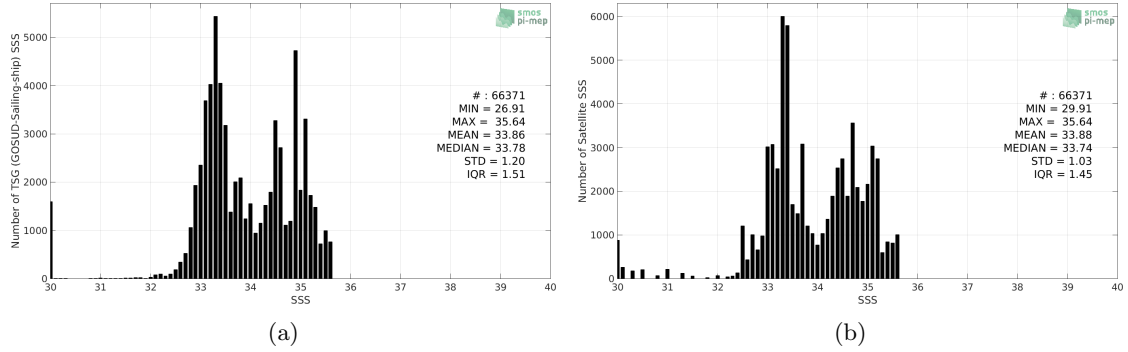
Figure 2: Histograms of SSS from TSG (GOSUD-Sailing-ship) (a) and SMAP SSS L4 OI v1 - Monthly (IPRC) (b) considering all match-up pairs per bins of 0.1 over the North Pacific Ocean Pi-MEP region and for the full satellite product period.
