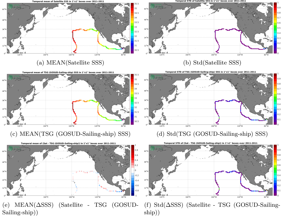
Figure 6: Temporal mean (left) and Std (right) of SSS from SMAP SSS L4 OI v1 - Monthly (IPRC) (top), TSG (GOSUD-Sailing-ship) (middle), and of \Delta\text{SSS} (Satellite - TSG (GOSUD-Sailing-ship)). Only match-up pairs are used to generate these maps.
