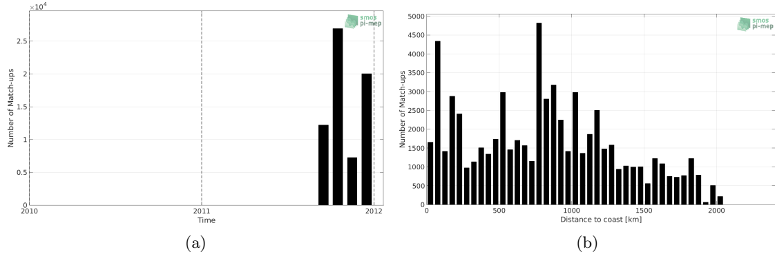
Figure 1: Number of match-ups between TSG (GOSUD-Sailing-ship) and SMAP SSS L4 OI v1 - Monthly (IPRC) SSS as a function of time (a) and as function of the distance to coast (b) over the North Pacific Ocean Pi-MEP region and for the full satellite product period.
