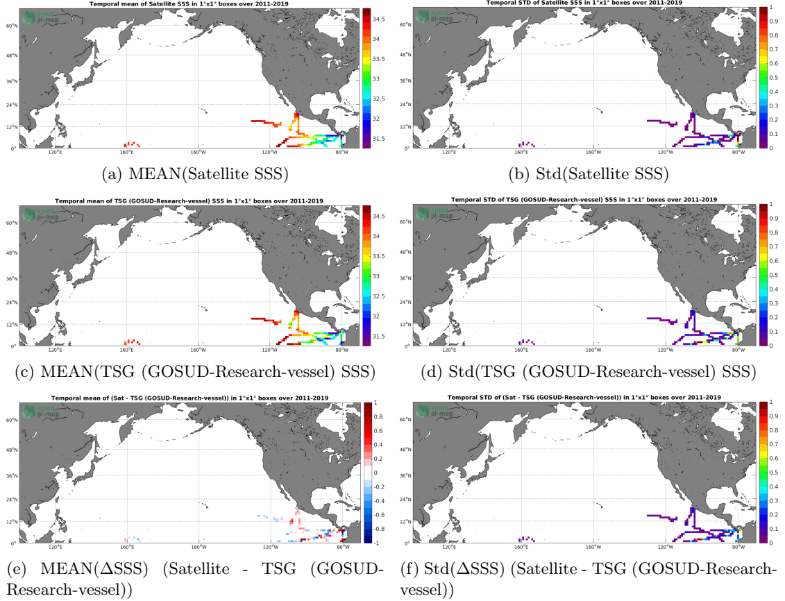
Figure 6: Temporal mean (left) and Std (right) of SSS from SMAP SSS L4 OI v1 - Monthly (IPRC) (top), TSG (GOSUD-Research-vessel) (middle), and of \Delta\text{SSS} (Satellite - TSG (GOSUD-Research-vessel)). Only match-up pairs are used to generate these maps.
