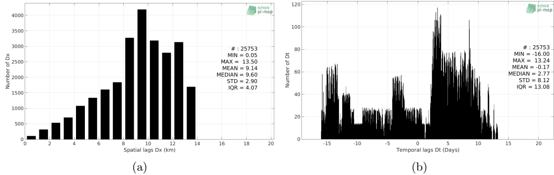
Figure 5: Histograms of the spatial (a) and temporal (b) lags between the location/time of the TSG (GOSUD-Research-vessel) measurement and the date of the corresponding SMAP SSS L4 OI v1 - Monthly (IPRC) SSS pixel.
