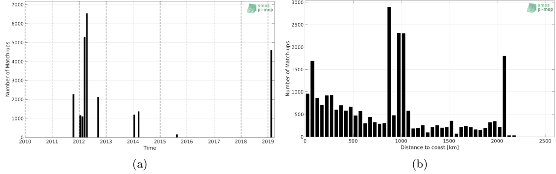
Figure 1: Number of match-ups between TSG (GOSUD-Research-vessel) and SMAP SSS L4 OI v1 - Monthly (IPRC) SSS as a function of time (a) and as function of the distance to coast (b) over the North Pacific Ocean Pi-MEP region and for the full satellite product period.
