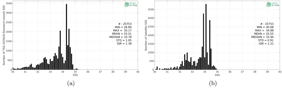
Figure 2: Histograms of SSS from TSG (GOSUD-Research-vessel) (a) and SMAP SSS L4 OI v1 - Monthly (IPRC) (b) considering all match-up pairs per bins of 0.1 over the North Pacific Ocean Pi-MEP region and for the full satellite product period.
