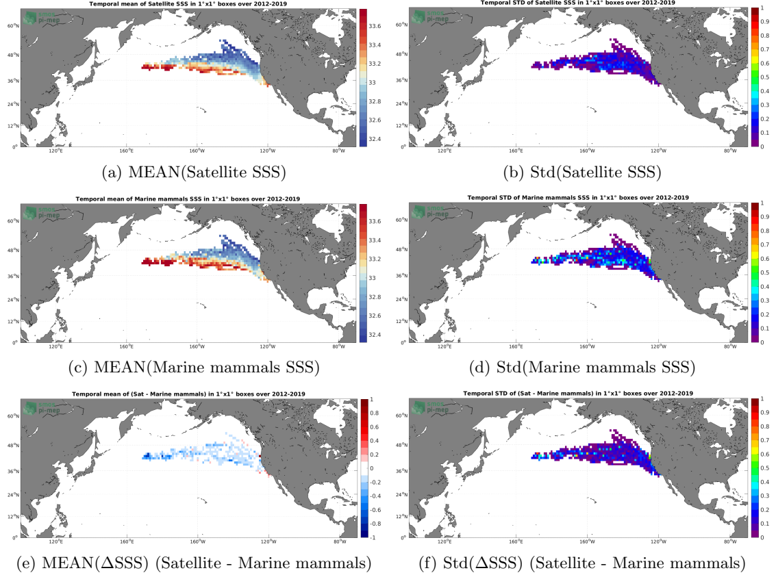
Figure 6: Temporal mean (left) and Std (right) of SSS from SMAP SSS L4 OI v1 - Monthly (IPRC) (top), Marine mammals (middle), and of \Delta SSS (Satellite - Marine mammals). Only match-up pairs are used to generate these maps.
