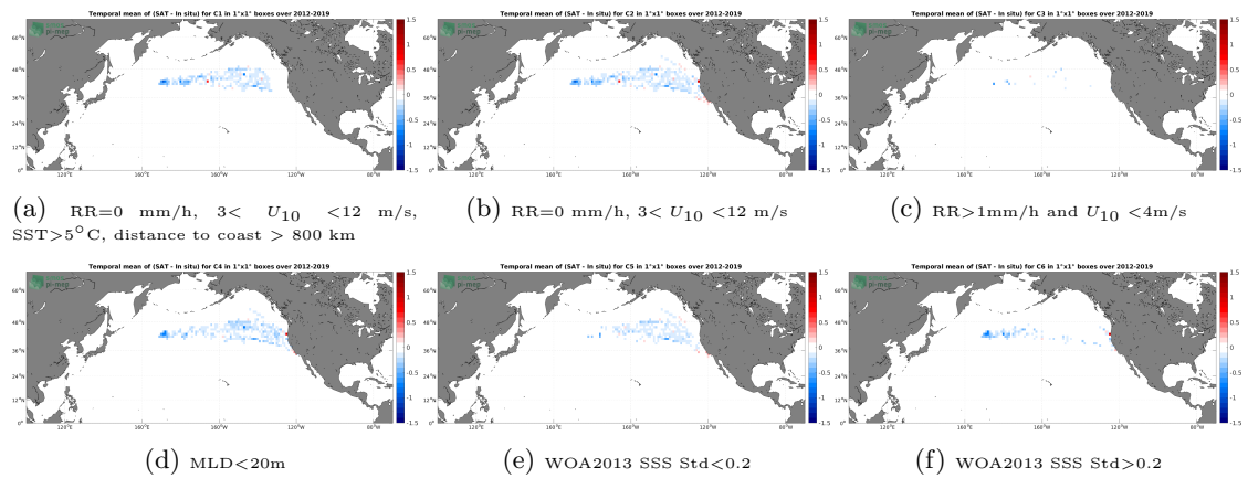
Figure 12: Temporal mean gridded over spatial boxes of size 1^\circ \times 1^\circ of \Delta SSS (SMAP SSS L4 OI v1 - Monthly (IPRC) - Marine mammals) for 6 different subdatasets corresponding to:RR=0 mm/h, 3 < U_{10} < 12 m/s, SST >5^\circ C, distance to coast > 800 km (a), RR=0 mm/h, 3 < U_{10} < 12 m/s (b), RR >1 mm/h and U_{10} < 4 m/s (c),MLD <20 m (d),WOA2013 SSS Std <0.2 (e),WOA2013 SSS Std >0.2 (f).
