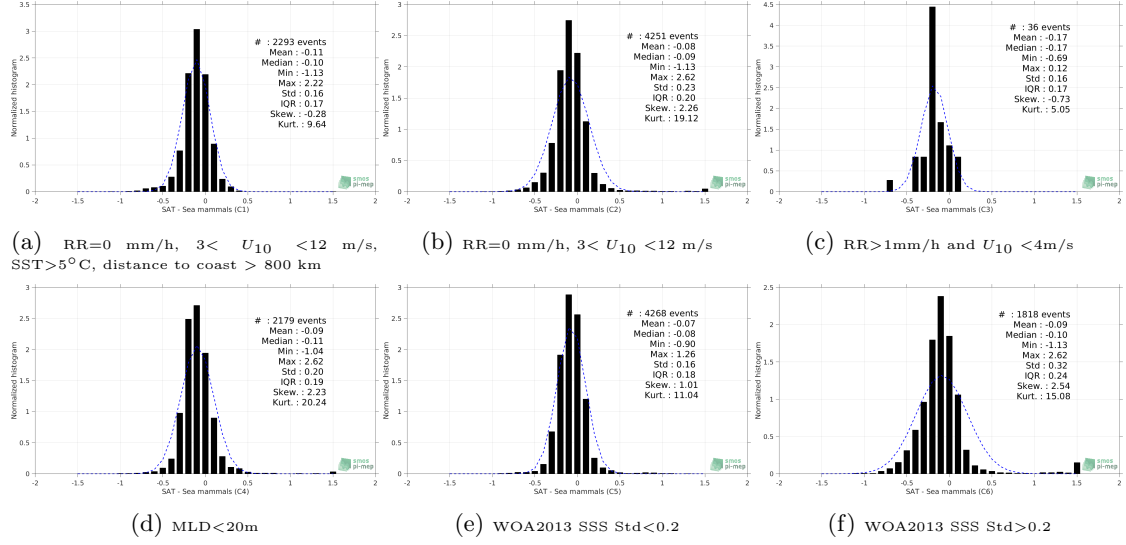
Figure 13: Normalized histogram of \Delta SSS (SMAP SSS L4 OI v1 - Monthly (IPRC) - Marine mammals) for 6 different subdatasets corresponding to: RR=0 mm/h, 3 < U_{10} < 12 m/s, SST>5°C, distance to coast > 800 km (a), RR=0 mm/h, 3 < U_{10} < 12 m/s (b), RR>1mm/h and U_{10} < 4 m/s (c), MLD<20m (d), WOA2013 SSS Std<0.2 (e), WOA2013 SSS Std>0.2 (f).
