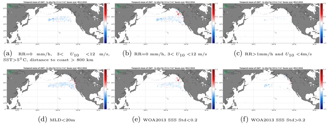
Figure 12: Temporal mean gridded over spatial boxes of size 1^\circ \times 1^\circ of \Delta SSS (SMAP SSS L4 OI v1 - Monthly (IPRC) - Marine mammals) for 6 different subdatasets corresponding to: RR=0 mm/h, 3 < U_{10} < 12 m/s, SST > 5^\circ C , distance to coast > 800 km (a), RR=0 mm/h, 3 < U_{10} < 12 m/s (b), RR > 1 mm/h and U_{10} < 4 m/s (c), MLD < 20 m (d), WOA2013 SSS Std < 0.2 (e), WOA2013 SSS Std > 0.2 (f).
