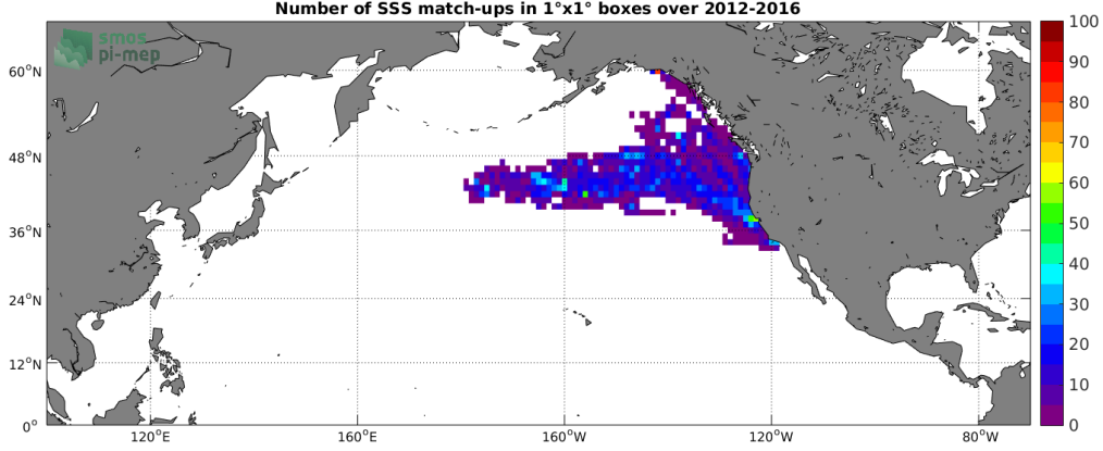
Figure 4: Number of SSS match-ups between Marine mammals SSS and the SMAP SSS L4 OI v1 - Monthly (IPRC) SSS product for the North Pacific Ocean Pi-MEP region over 1^\circ \times 1^\circ boxes and for the full satellite product period.
