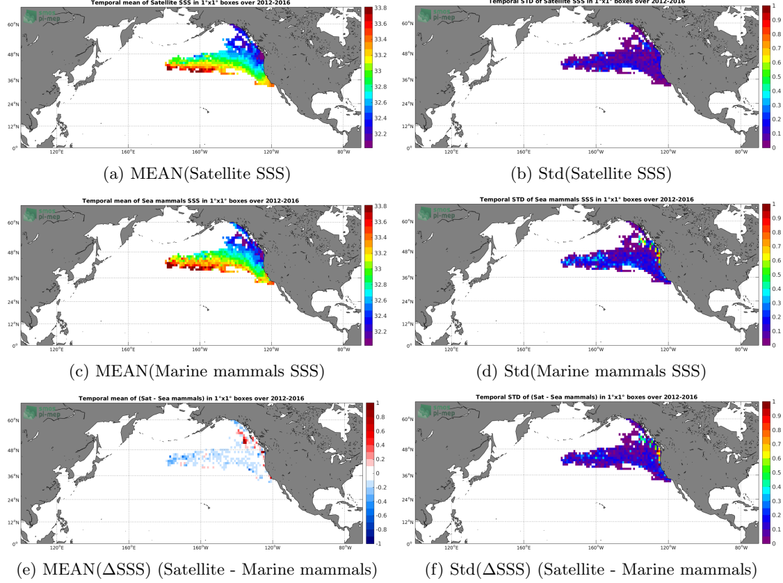
Figure 6: Temporal mean (left) and Std (right) of SSS from SMAP SSS L4 OI v1 - Monthly (IPRC) (top), Marine mammals (middle), and of \Delta\text{SSS} (Satellite - Marine mammals). Only match-up pairs are used to generate these maps.
