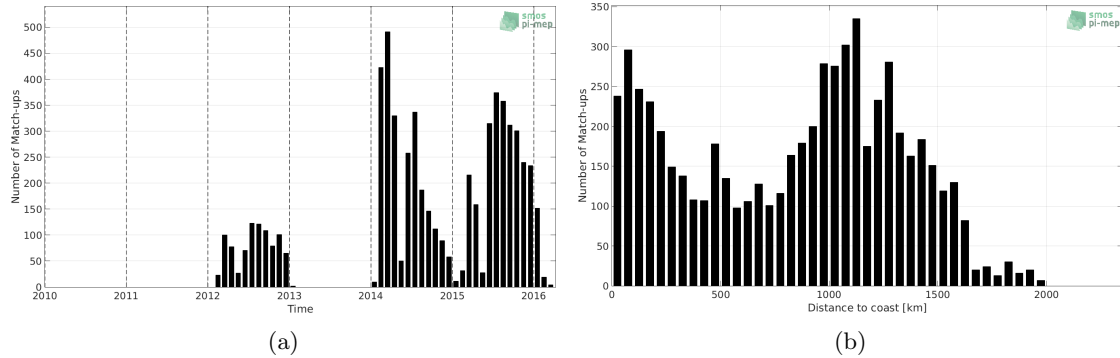
Figure 1: Number of match-ups between Marine mammals and SMAP SSS L4 OI v1 - Monthly (IPRC) SSS as a function of time (a) and as function of the distance to coast (b) over the North Pacific Ocean Pi-MEP region and for the full satellite product period.
