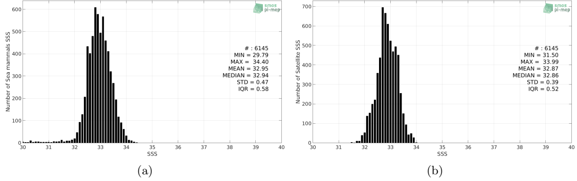
Figure 2: Histograms of SSS from Marine mammals (a) and SMAP SSS L4 OI v1 - Monthly (IPRC) (b) considering all match-up pairs per bins of 0.1 over the North Pacific Ocean Pi-MEP region and for the full satellite product period.
