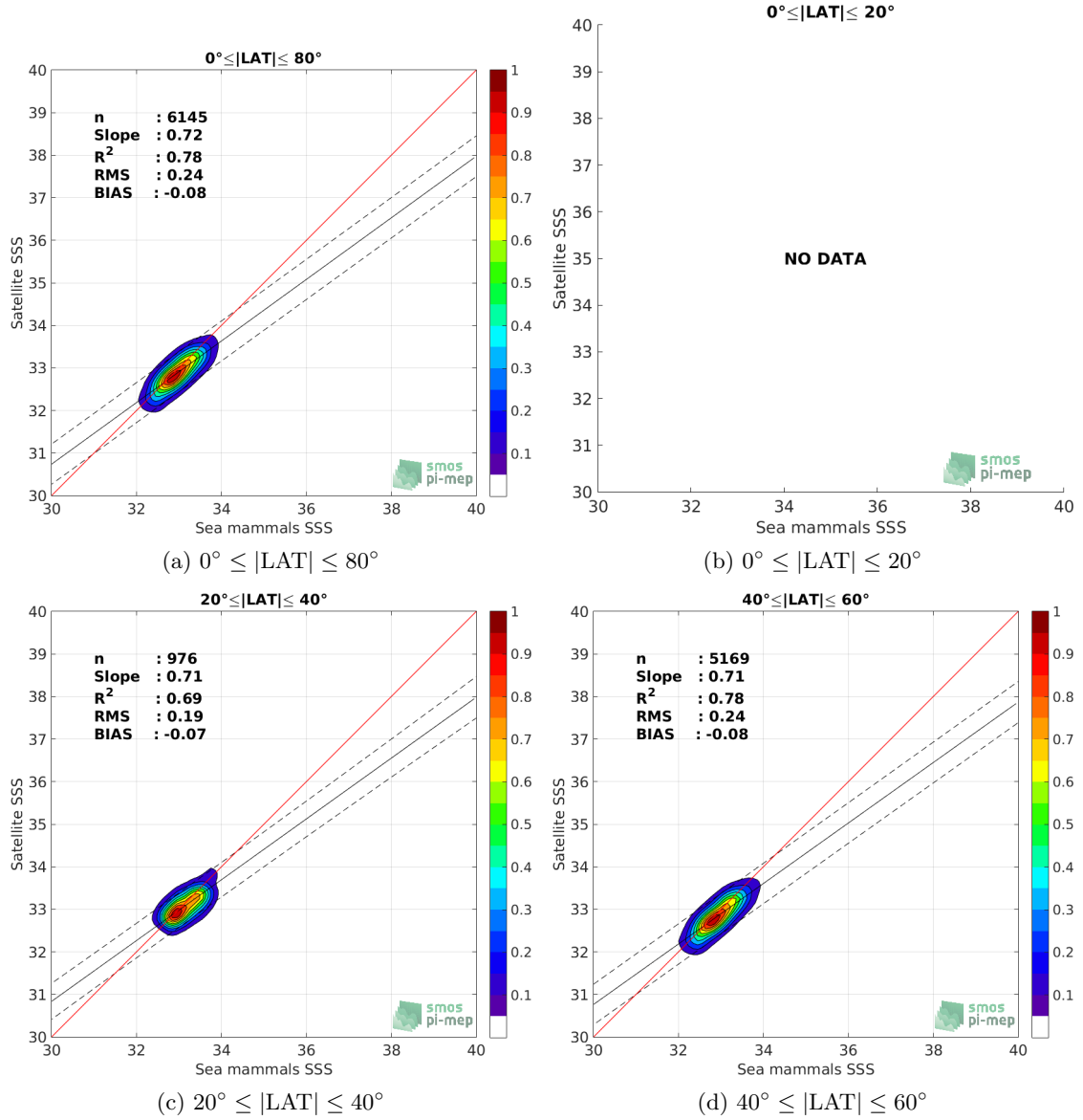
Figure 9: Contour maps of the concentration of SMAP SSS L4 OI v1 - Monthly (IPRC) SSS (y-axis) versus Marine mammals SSS (x-axis) at match-up pairs for different latitude bands. For each plot, the red line shows x=y . The black thin and dashed lines indicate a linear fit through the data cloud and the \pm 95\% confidence levels, respectively. The number match-up pairs n , the slope and R^2 coefficient of the linear fit, the root mean square (RMS) and the mean bias between satellite and in situ data are indicated for each latitude band in each plots.
