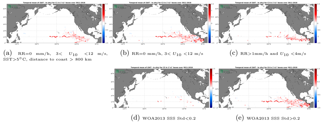
Figure 11: Temporal mean gridded over spatial boxes of size 1^\circ \times 1^\circ of \Delta SSS (SMAP SSS L4 OI v1 - Monthly (IPRC) - Surface drifters) for 5 different subdatasets corresponding to: RR=0 mm/h, 3 < U_{10} < 12 m/s, SST > 5^\circ C , distance to coast > 800 km (a), RR=0 mm/h, 3 < U_{10} < 12 m/s (b), RR > 1 mm/h and U_{10} < 4 m/s (c), WOA2013 SSS Std < 0.2 (d), WOA2013 SSS Std > 0.2 (e).
