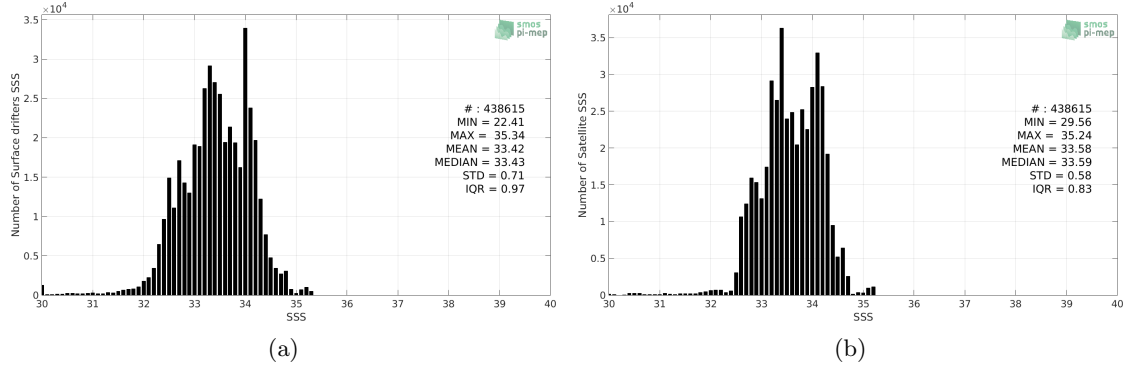
Figure 2: Histograms of SSS from Surface drifters (a) and SMAP SSS L4 OI v1 - Monthly (IPRC) (b) considering all match-up pairs per bins of 0.1 over the North Pacific Ocean Pi-MEP region and for the full satellite product period.
