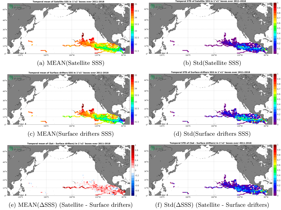
Figure 5: Temporal mean (left) and Std (right) of SSS from SMAP SSS L4 OI v1 - Monthly (IPRC) (top), Surface drifters (middle), and of \Delta SSS (Satellite - Surface drifters). Only match-up pairs are used to generate these maps.
