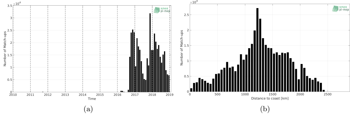
Figure 1: Number of match-ups between Surface drifters and SMAP SSS L4 OI v1 - Monthly (IPRC) SSS as a function of time (a) and as function of the distance to coast (b) over the North Pacific Ocean Pi-MEP region and for the full satellite product period.
