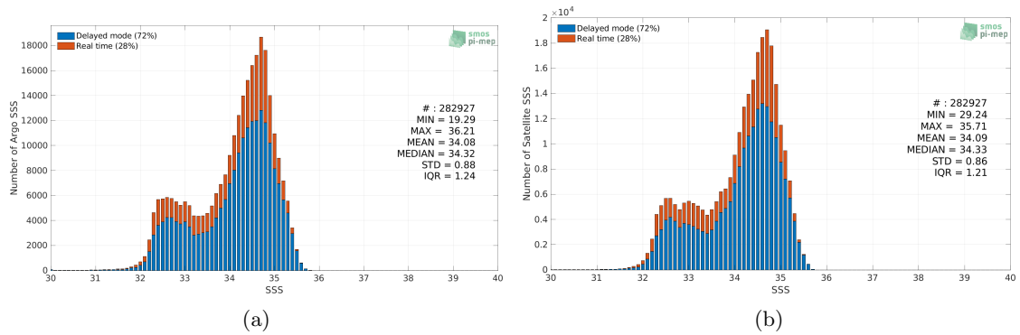
Figure 2: Histograms of SSS from Argo (a) and SMAP SSS L4 OI v1 - Monthly (IPRC) (b) considering all match-up pairs per bins of 0.1 over the North Pacific Ocean Pi-MEP region and for the full satellite product period.
