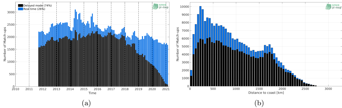
Figure 1: Number of match-ups between Argo and SMAP SSS L4 OI v1 - Monthly (IPRC) SSS as a function of time (a) and as function of the distance to coast (b) over the North Pacific Ocean Pi-MEP region and for the full satellite product period.
