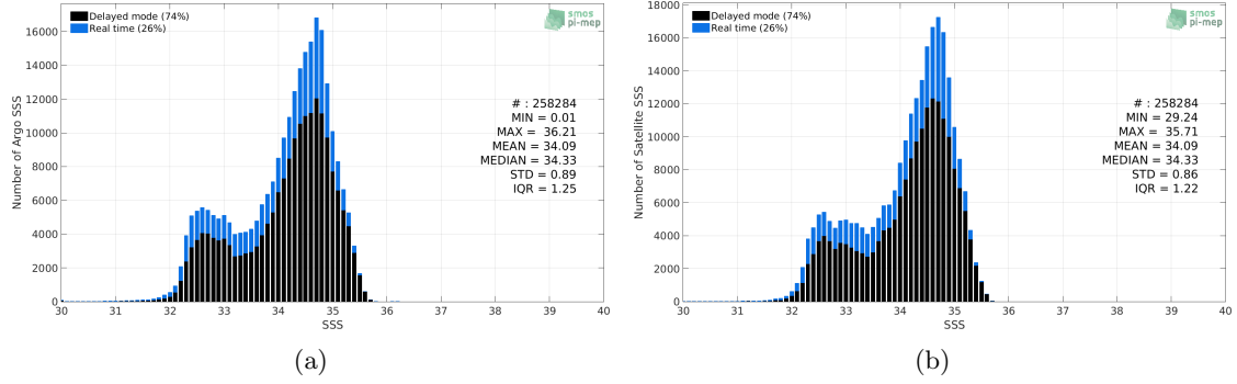
Figure 2: Histograms of SSS from Argo (a) and SMAP SSS L4 OI v1 - Monthly (IPRC) (b) considering all match-up pairs per bins of 0.1 over the North Pacific Ocean Pi-MEP region and for the full satellite product period.
