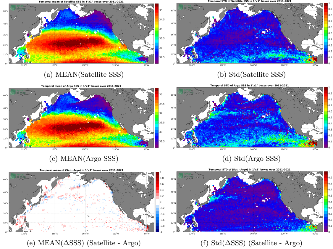
Figure 6: Temporal mean (left) and Std (right) of SSS from SMAP SSS L4 OI v1 - Monthly (IPRC) (top), Argo (middle), and of \Delta\text{SSS} (Satellite - Argo). Only match-up pairs are used to generate these maps.
