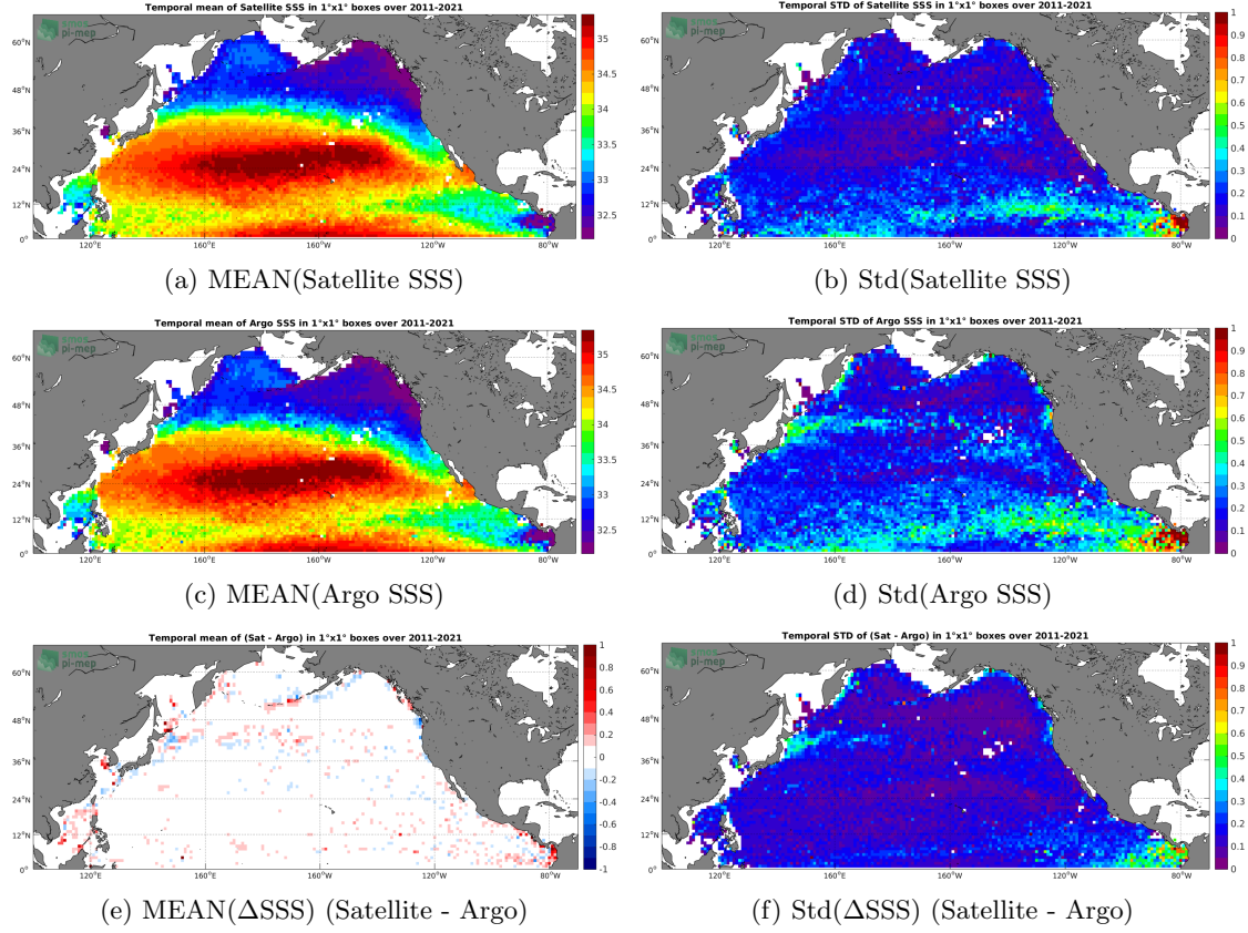
Figure 6: Temporal mean (left) and Std (right) of SSS from SMAP SSS L4 OI v1 - Monthly (IPRC) (top), Argo (middle), and of \Delta SSS (Satellite - Argo). Only match-up pairs are used to generate these maps.
