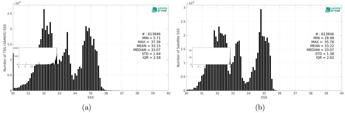
Figure 3: Histograms of SSS from TSG (SAMOS) (a) and SMAP SSS L4 OI v3 - Monthly (ESR) (b) considering all match-up pairs per bins of 0.1 over the North Pacific Ocean Pi-MEP region and for the full satellite product period.
