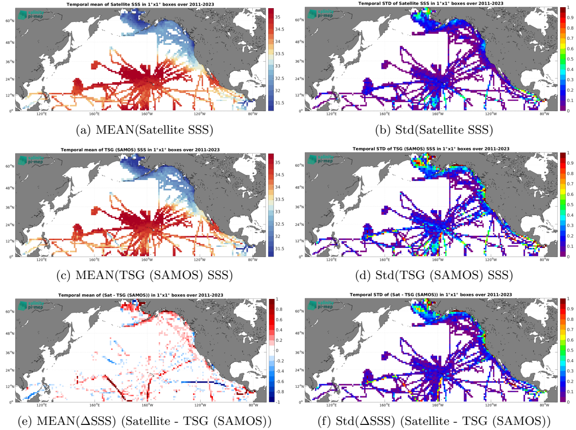
Figure 7: Temporal mean (left) and Std (right) of SSS from SMAP SSS L4 OI v3 - Monthly (ESR) (top), TSG (SAMOS) (middle), and of \Delta\text{SSS} (Satellite - TSG (SAMOS)). Only match-up pairs are used to generate these maps.
