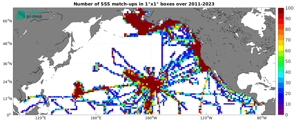
Figure 5: Number of SSS match-ups between TSG (SAMOS) SSS and the SMAP SSS L4 OI v3 - Monthly (ESR) SSS product for the North Pacific Ocean Pi-MEP region over 1^\circ \times 1^\circ boxes and for the full satellite product period.
