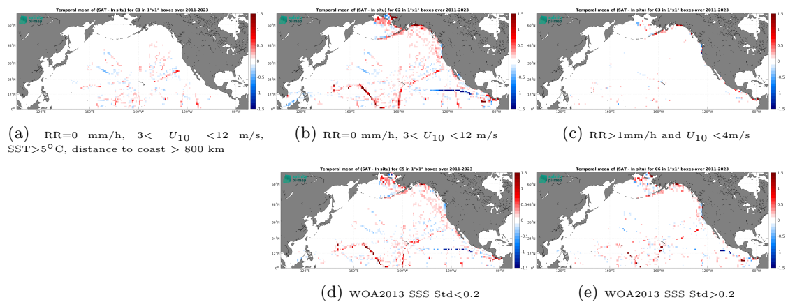
Figure 14: Temporal mean gridded over spatial boxes of size 1^\circ \times 1^\circ of \Delta\text{SSS} (SMAP SSS L4 OI v3 - Monthly (ESR) - TSG (SAMOS)) for 5 different subdatasets corresponding to: RR=0 mm/h, 3 < U_{10} < 12 m/s, SST > 5°C, distance to coast > 800 km (a), RR=0 mm/h, 3 < U_{10} < 12 m/s (b), RR > 1mm/h and U_{10} < 4 m/s (c), WOA2013 SSS Std < 0.2 (d), WOA2013 SSS Std > 0.2 (e).
