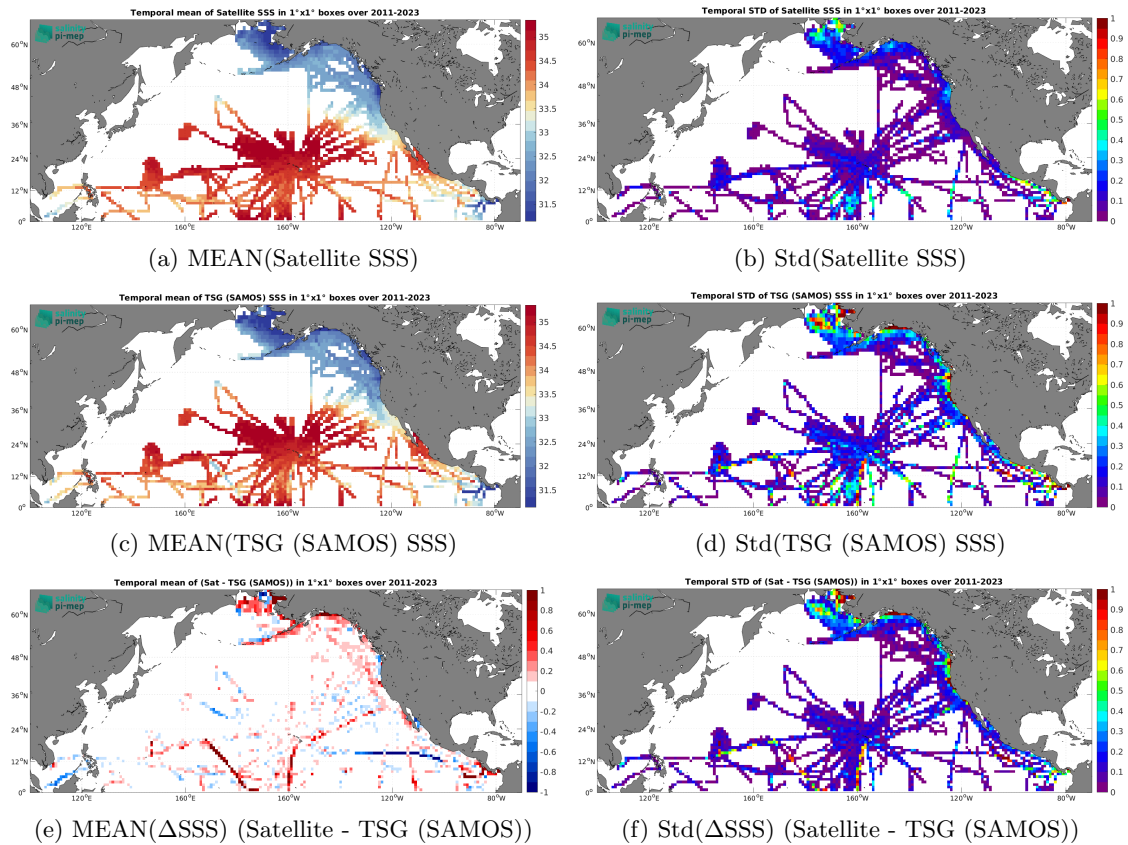
Figure 7: Temporal mean (left) and Std (right) of SSS from SMAP SSS L4 OI v3 - Monthly (ESR) (top), TSG (SAMOS) (middle), and of \Delta SSS (Satellite - TSG (SAMOS)). Only match-up pairs are used to generate these maps.
