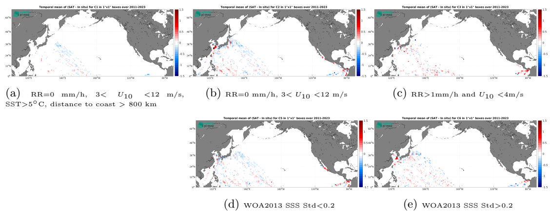
Figure 14: Temporal mean gridded over spatial boxes of size 1^\circ \times 1^\circ of \Delta\text{SSS} (SMAP SSS L4 OI v3 - Monthly (ESR) - TSG (LEGOS-DM)) for 5 different subdatasets corresponding to: RR=0 mm/h, 3 < U_{10} < 12 m/s, SST > 5°C, distance to coast > 800 km (a), RR=0 mm/h, 3 < U_{10} < 12 m/s (b), RR > 1 mm/h and U_{10} < 4 m/s (c), WOA2013 SSS Std < 0.2 (d), WOA2013 SSS Std > 0.2 (e).
