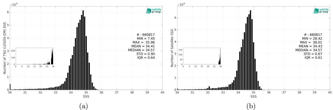
Figure 3: Histograms of SSS from TSG (LEGOS-DM) (a) and SMAP SSS L4 OI v3 - Monthly (ESR) (b) considering all match-up pairs per bins of 0.1 over the North Pacific Ocean Pi-MEP region and for the full satellite product period.
