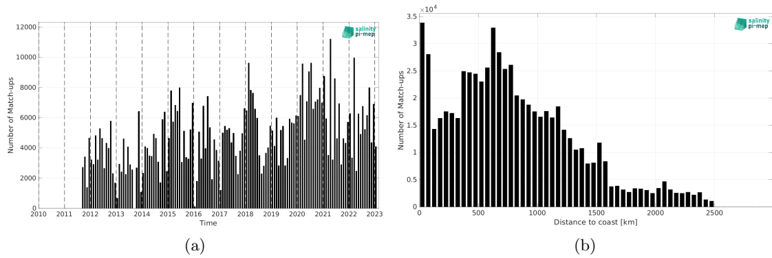
Figure 2: Number of match-ups between TSG (LEGOS-DM) and SMAP SSS L4 OI v3 - Monthly (ESR) SSS as a function of time (a) and as function of the distance to coast (b) over the North Pacific Ocean Pi-MEP region and for the full satellite product period.
