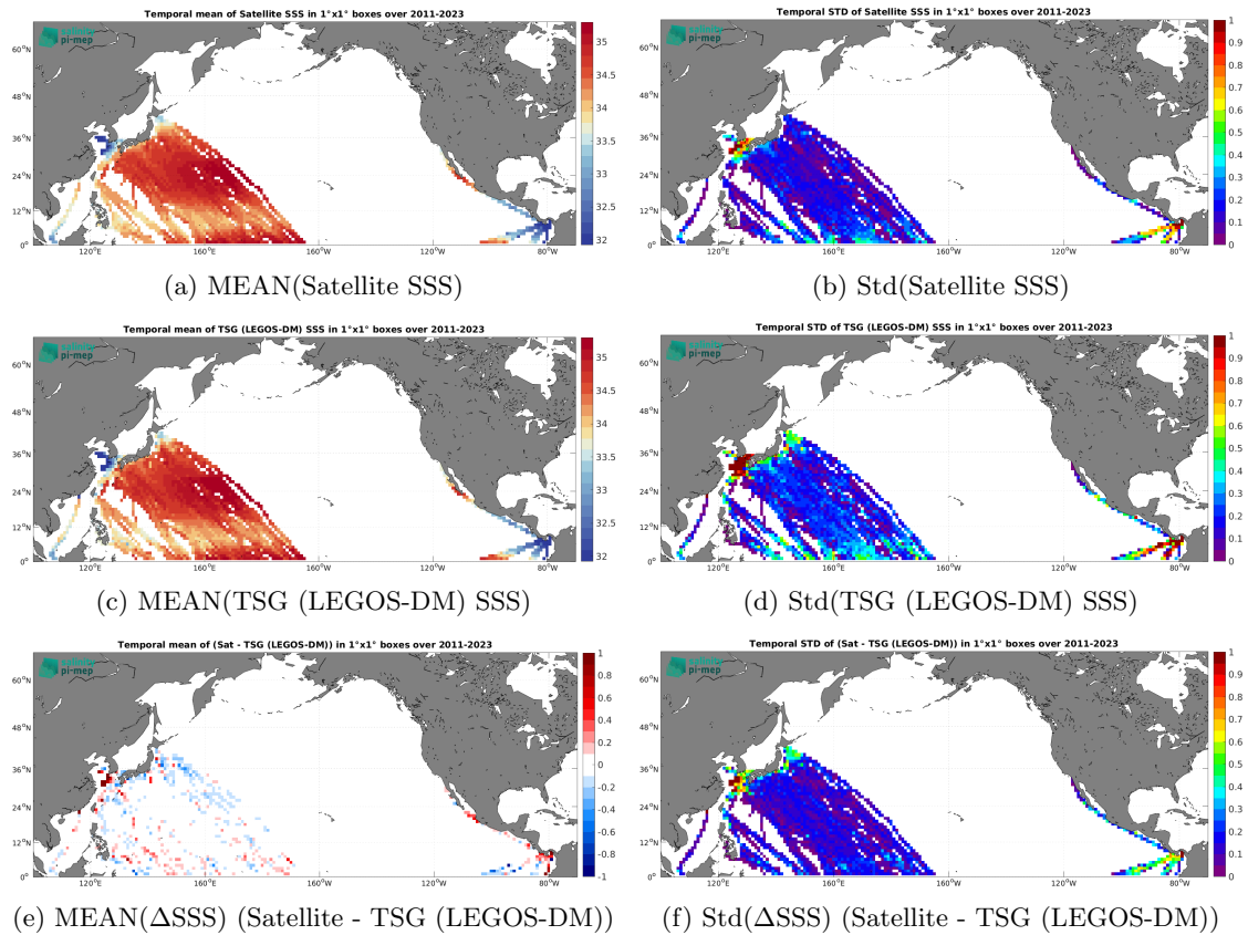
Figure 7: Temporal mean (left) and Std (right) of SSS from SMAP SSS L4 OI v3 - Monthly (ESR) (top), TSG (LEGOS-DM) (middle), and of \Delta SSS (Satellite - TSG (LEGOS-DM)). Only match-up pairs are used to generate these maps.
