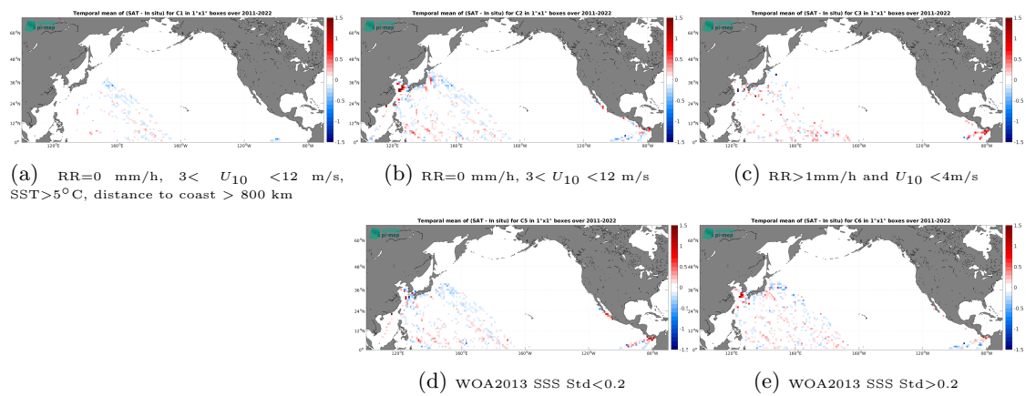
Figure 14: Temporal mean gridded over spatial boxes of size 1^\circ \times 1^\circ of \Delta SSS (SMAP SSS L4 OI v3 - Monthly (ESR) - TSG (LEGOS-DM)) for 5 different subdatasets corresponding to: RR=0 mm/h, 3 < U_{10} < 12 m/s, SST > 5°C, distance to coast > 800 km (a), RR=0 mm/h, 3 < U_{10} < 12 m/s (b), RR > 1mm/h and U_{10} < 4 m/s (c), WOA2013 SSS Std < 0.2 (d), WOA2013 SSS Std > 0.2 (e).
