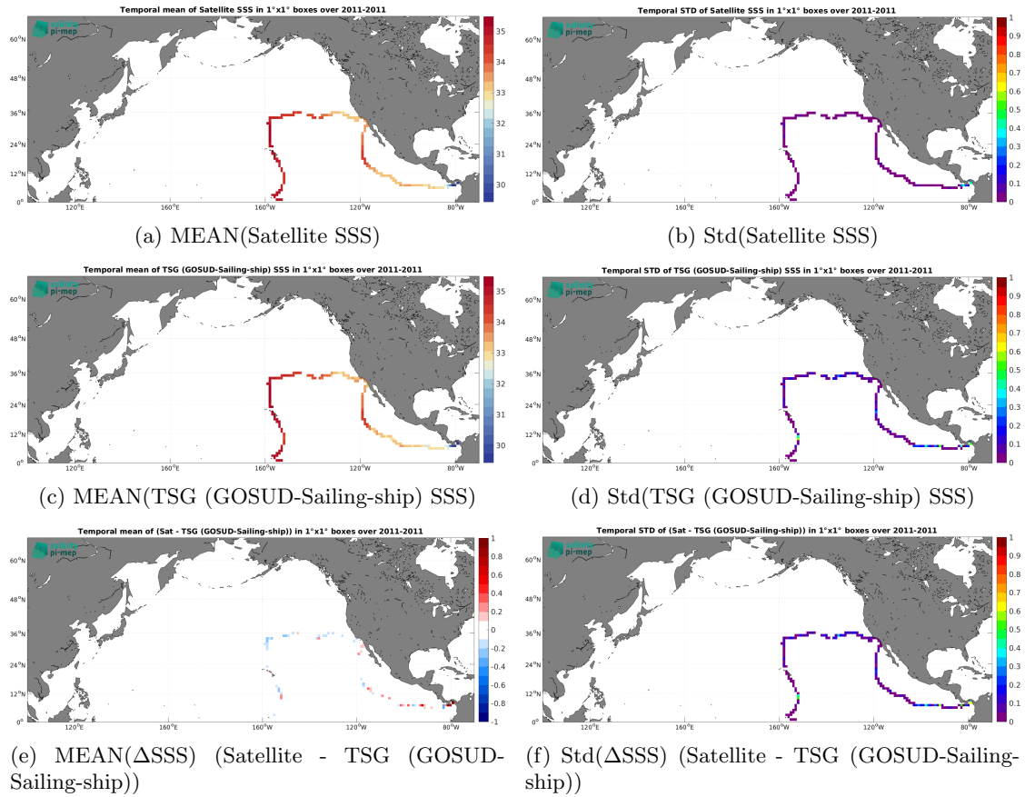
Figure 7: Temporal mean (left) and Std (right) of SSS from SMAP SSS L4 OI v3 - Monthly (ESR) (top), TSG (GOSUD-Sailing-ship) (middle), and of \Delta SSS (Satellite - TSG (GOSUD-Sailing-ship)). Only match-up pairs are used to generate these maps.
