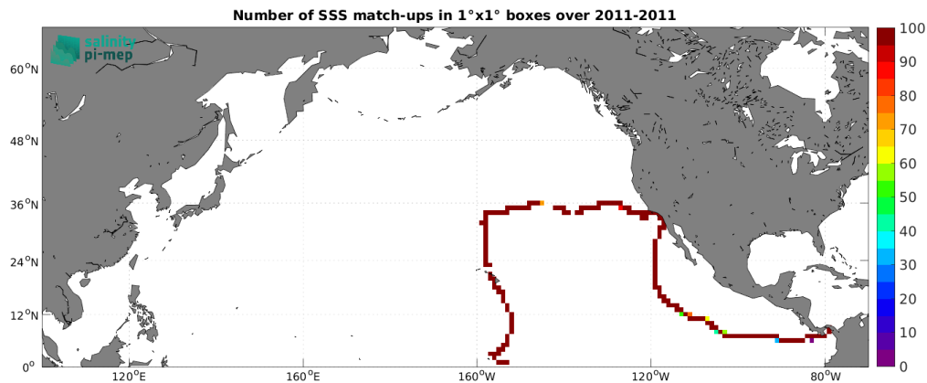
Figure 5: Number of SSS match-ups between TSG (GOSUD-Sailing-ship) SSS and the SMAP SSS L4 OI v3 - Monthly (ESR) SSS product for the North Pacific Ocean Pi-MEP region over 1^\circ \times 1^\circ boxes and for the full satellite product period.
