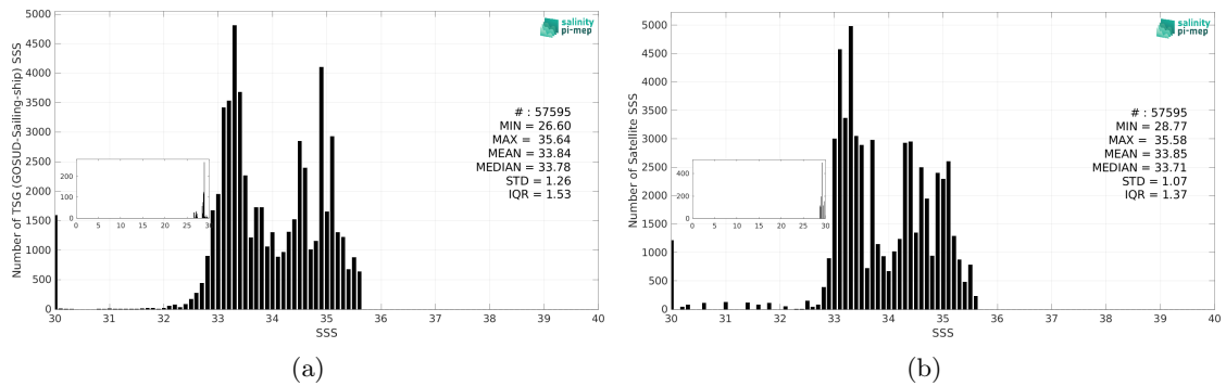
Figure 3: Histograms of SSS from TSG (GOSUD-Sailing-ship) (a) and SMAP SSS L4 OI v3 - Monthly (ESR) (b) considering all match-up pairs per bins of 0.1 over the North Pacific Ocean Pi-MEP region and for the full satellite product period.
