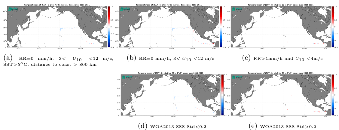
Figure 14: Temporal mean gridded over spatial boxes of size 1^\circ \times 1^\circ of \Delta\text{SSS} (SMAP SSS L4 OI v3 - Monthly (ESR) - TSG (GOSUD-Sailing-ship)) for 5 different subdatasets corresponding to:RR=0 mm/h, 3 < U_{10} < 12 m/s, SST>5°C, distance to coast > 800 km (a), RR=0 mm/h, 3 < U_{10} < 12 m/s (b), RR>1mm/h and U_{10} < 4 m/s (c), WOA2013 SSS Std<0.2 (d), WOA2013 SSS Std>0.2 (e).
