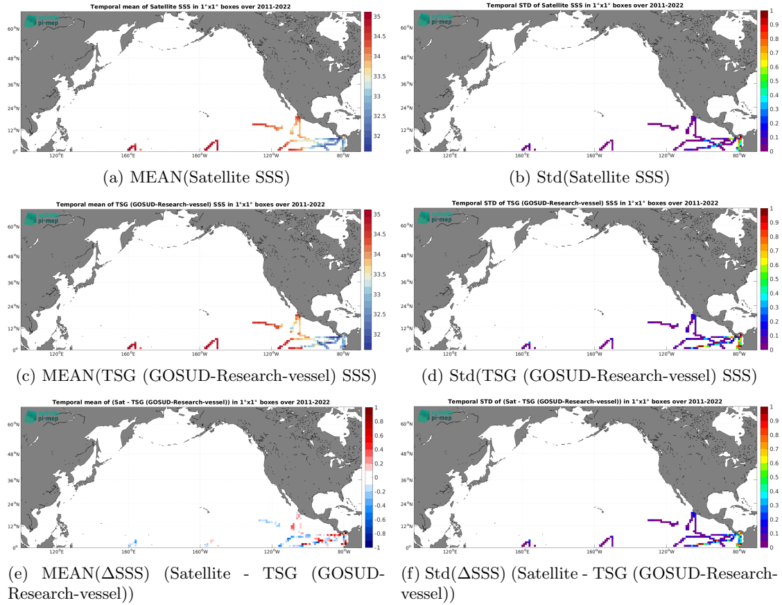
Figure 7: Temporal mean (left) and Std (right) of SSS from SMAP SSS L4 OI v3 - Monthly (ESR) (top), TSG (GOSUD-Research-vessel) (middle), and of \Delta SSS (Satellite - TSG (GOSUD-Research-vessel)). Only match-up pairs are used to generate these maps.
