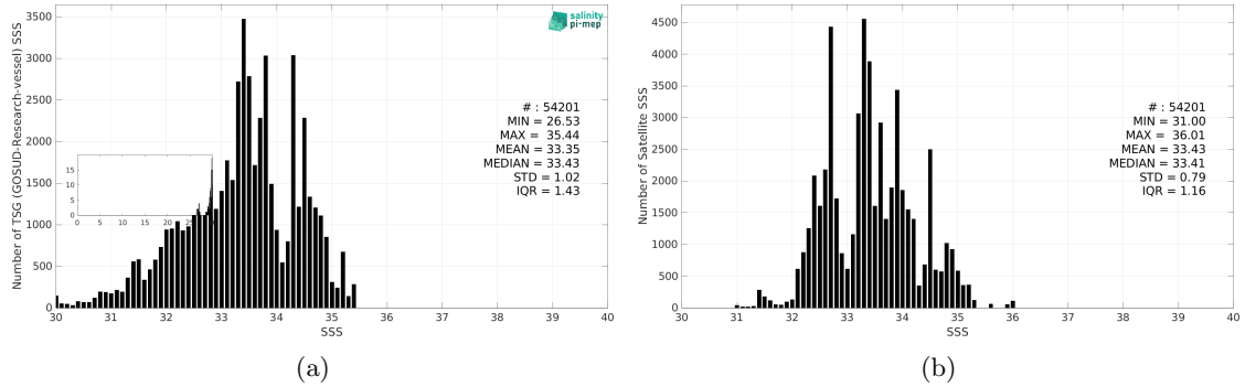
Figure 3: Histograms of SSS from TSG (GOSUD-Research-vessel) (a) and SMAP SSS L4 OI v3 - Monthly (ESR) (b) considering all match-up pairs per bins of 0.1 over the North Pacific Ocean Pi-MEP region and for the full satellite product period.
