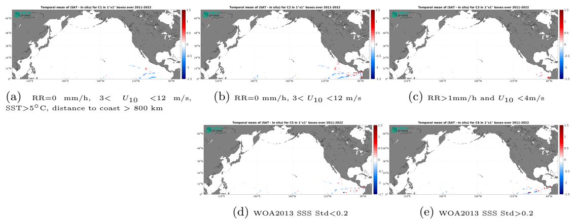
Figure 14: Temporal mean gridded over spatial boxes of size 1^\circ \times 1^\circ of \Delta\text{SSS} (SMAP SSS L4 OI v3 - Monthly (ESR) - TSG (GOSUD-Research-vessel)) for 5 different subdatasets corresponding to:RR=0 mm/h, 3 < U_{10} < 12 m/s, SST>5°C, distance to coast > 800 km (a), RR=0 mm/h, 3 < U_{10} < 12 m/s (b), RR>1mm/h and U_{10} < 4 m/s (c), WOA2013 SSS Std<0.2 (d), WOA2013 SSS Std>0.2 (e).
