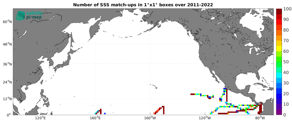
Figure 5: Number of SSS match-ups between TSG (GOSUD-Research-vessel) SSS and the SMAP SSS L4 OI v3 - Monthly (ESR) SSS product for the North Pacific Ocean Pi-MEP region over 1^\circ \times 1^\circ boxes and for the full satellite product period.
