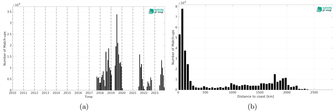
Figure 2: Number of match-ups between Saldrone and SMAP SSS L4 OI v3 - Monthly (ESR) SSS as a function of time (a) and as function of the distance to coast (b) over the North Pacific Ocean Pi-MEP region and for the full satellite product period.
