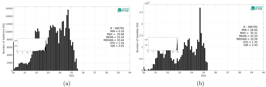
Figure 3: Histograms of SSS from Saldrone (a) and SMAP SSS L4 OI v3 - Monthly (ESR) (b) considering all match-up pairs per bins of 0.1 over the North Pacific Ocean Pi-MEP region and for the full satellite product period.
