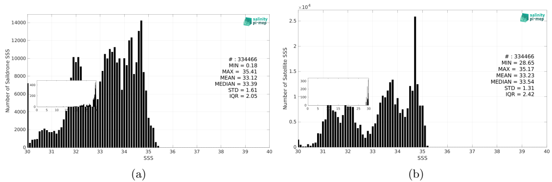
Figure 3: Histograms of SSS from Sailldrone (a) and SMAP SSS L4 OI v3 - Monthly (ESR) (b) considering all match-up pairs per bins of 0.1 over the North Pacific Ocean Pi-MEP region and for the full satellite product period.
