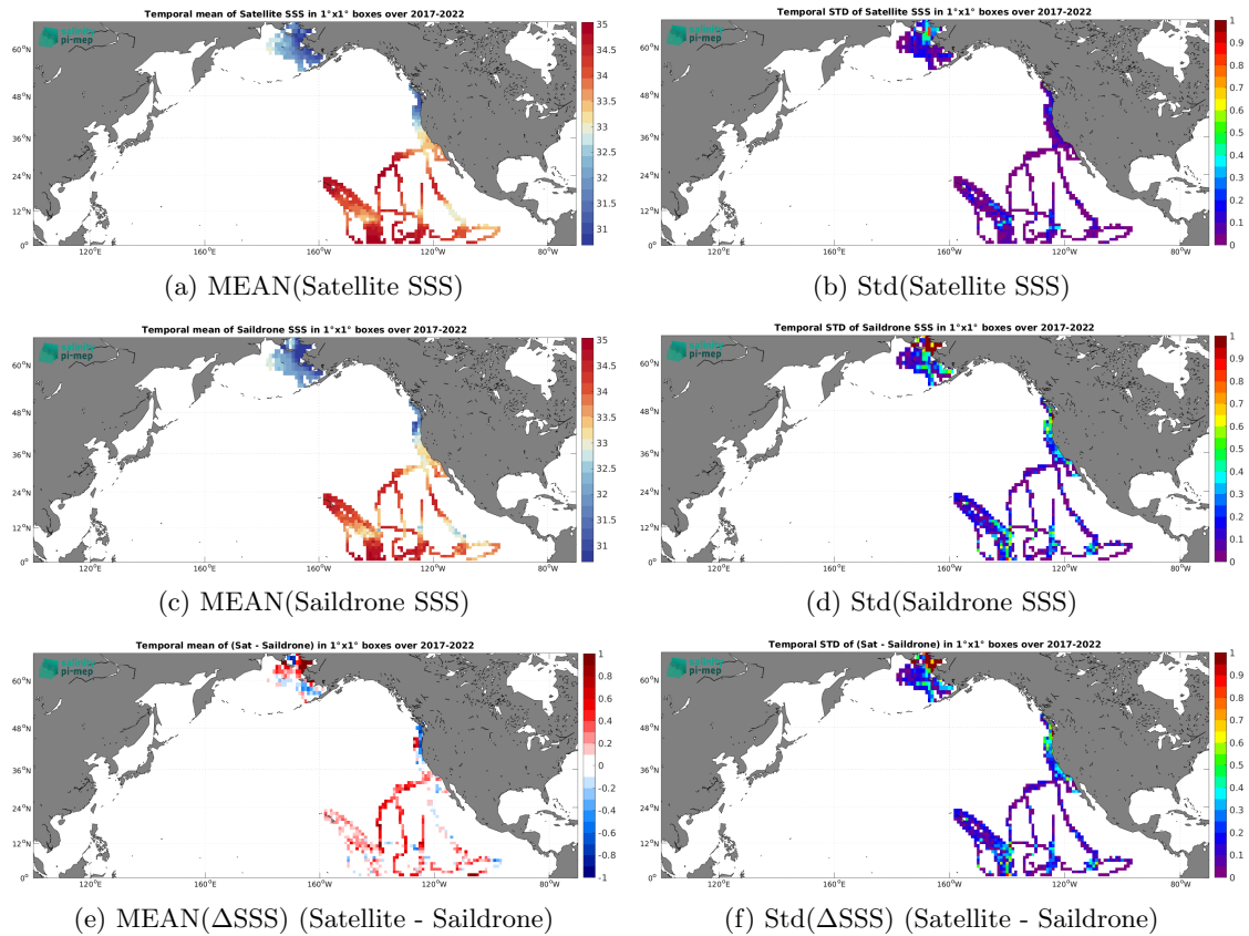
Figure 7: Temporal mean (left) and Std (right) of SSS from SMAP SSS L4 OI v3 - Monthly (ESR) (top), Saildrone (middle), and of \Delta SSS (Satellite - Saildrone). Only match-up pairs are used to generate these maps.
