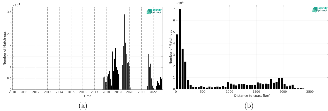
Figure 2: Number of match-ups between Sailldrone and SMAP SSS L4 OI v3 - Monthly (ESR) SSS as a function of time (a) and as function of the distance to coast (b) over the North Pacific Ocean Pi-MEP region and for the full satellite product period.
