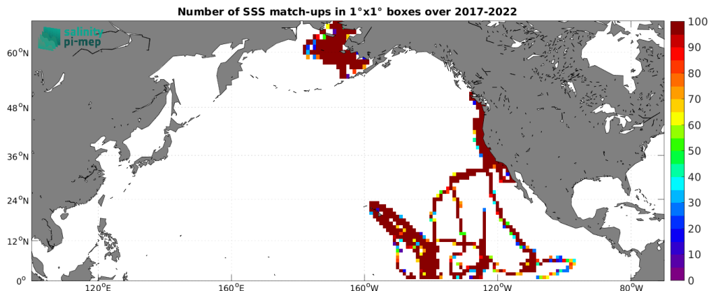
Figure 5: Number of SSS match-ups between Saildrone SSS and the SMAP SSS L4 OI v3 - Monthly (ESR) SSS product for the North Pacific Ocean Pi-MEP region over 1^\circ \times 1^\circ boxes and for the full satellite product period.
