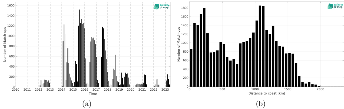
Figure 2: Number of match-ups between Marine mammals and SMAP SSS L4 OI v3 - Monthly (ESR) SSS as a function of time (a) and as function of the distance to coast (b) over the North Pacific Ocean Pi-MEP region and for the full satellite product period.
