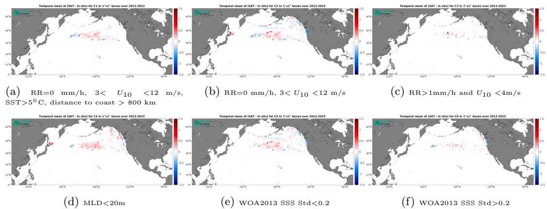
Figure 14: Temporal mean gridded over spatial boxes of size 1^\circ \times 1^\circ of \Delta SSS (SMAP SSS L4 OI v3 - Monthly (ESR) - Marine mammals) for 6 different subdatasets corresponding to:RR=0 mm/h, 3 < U_{10} < 12 m/s, SST>5°C, distance to coast > 800 km (a), RR=0 mm/h, 3 < U_{10} < 12 m/s (b), RR>1mm/h and U_{10} < 4 m/s (c),MLD<20m (d),WOA2013 SSS Std<0.2 (e),WOA2013 SSS Std>0.2 (f).
