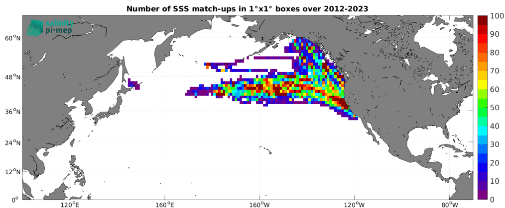
Figure 5: Number of SSS match-ups between Marine mammals SSS and the SMAP SSS L4 OI v3 - Monthly (ESR) SSS product for the North Pacific Ocean Pi-MEP region over 1^\circ \times 1^\circ boxes and for the full satellite product period.
