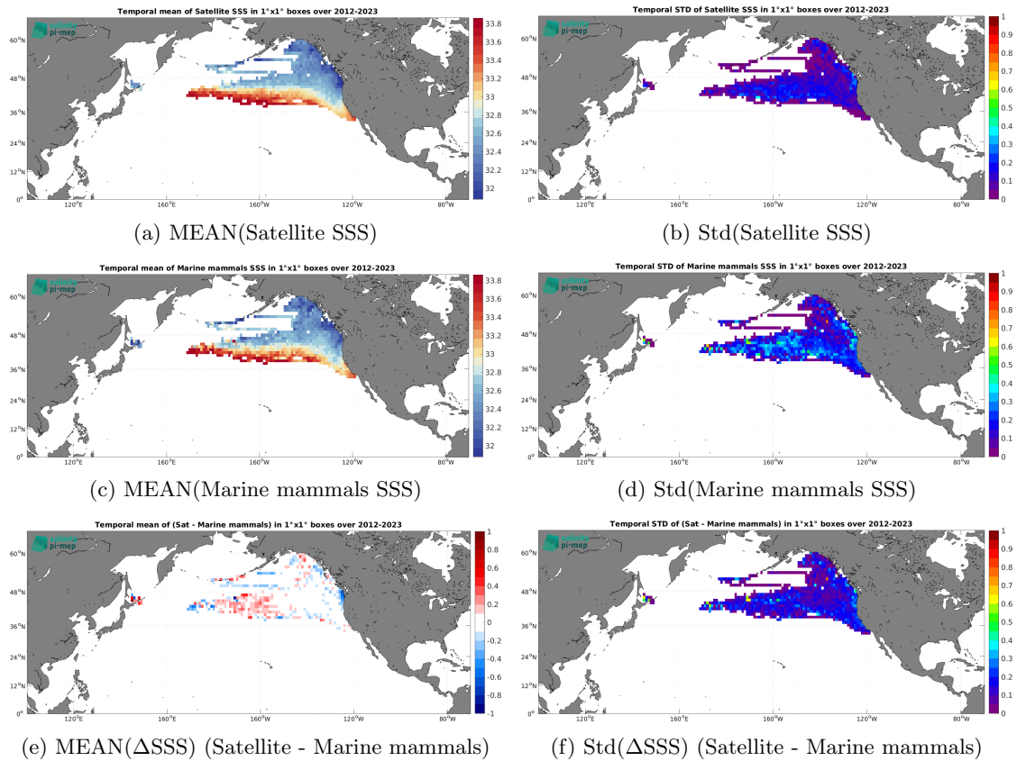
Figure 7: Temporal mean (left) and Std (right) of SSS from SMAP SSS L4 OI v3 - Monthly (ESR) (top), Marine mammals (middle), and of \Delta SSS (Satellite - Marine mammals). Only match-up pairs are used to generate these maps.
