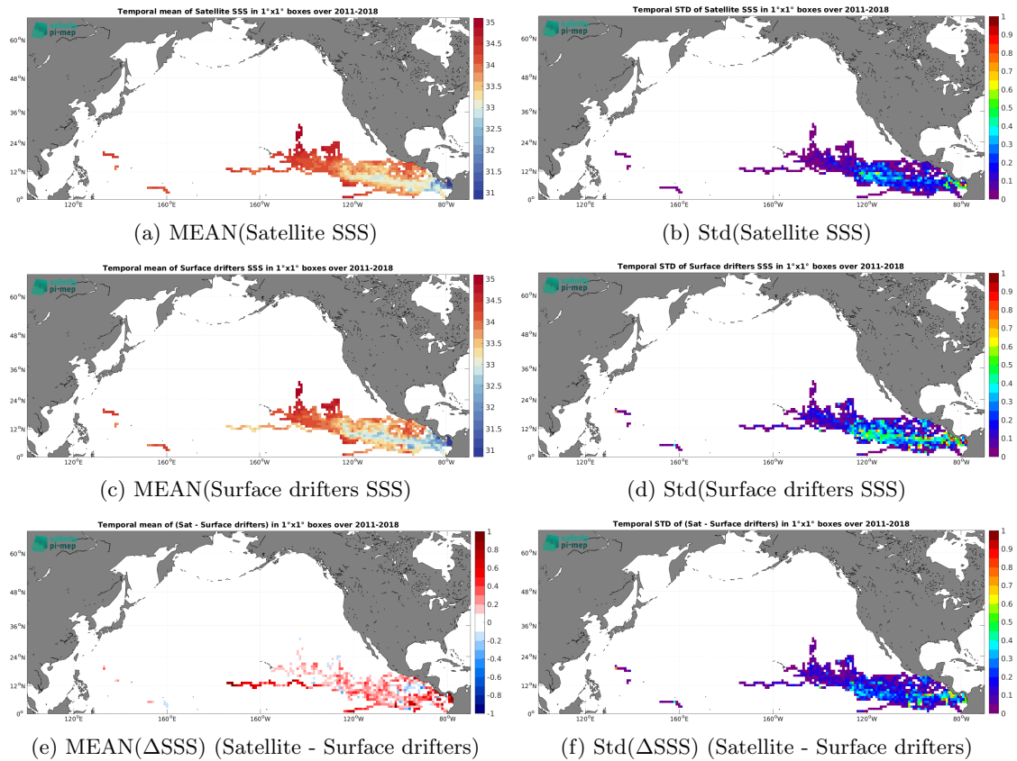
Figure 6: Temporal mean (left) and Std (right) of SSS from SMAP SSS L4 OI v3 - Monthly (ESR) (top), Surface drifters (middle), and of \Delta SSS (Satellite - Surface drifters). Only match-up pairs are used to generate these maps.
