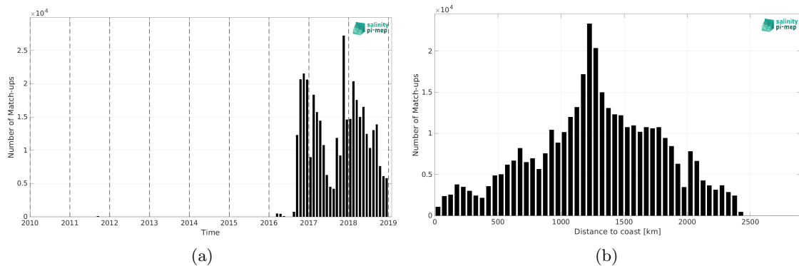
Figure 2: Number of match-ups between Surface drifters and SMAP SSS L4 OI v3 - Monthly (ESR) SSS as a function of time (a) and as function of the distance to coast (b) over the North Pacific Ocean Pi-MEP region and for the full satellite product period.
