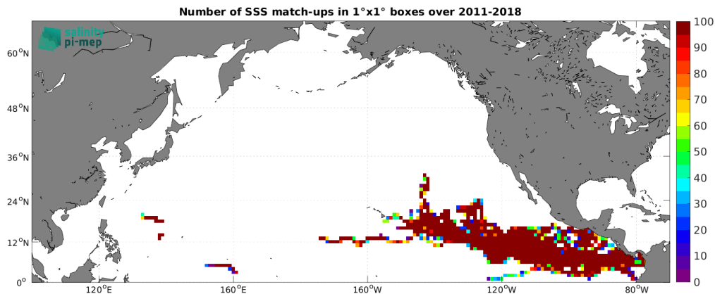
Figure 4: Number of SSS match-ups between Surface drifters SSS and the SMAP SSS L4 OI v3 - Monthly (ESR) SSS product for the North Pacific Ocean Pi-MEP region over 1^\circ \times 1^\circ boxes and for the full satellite product period.
