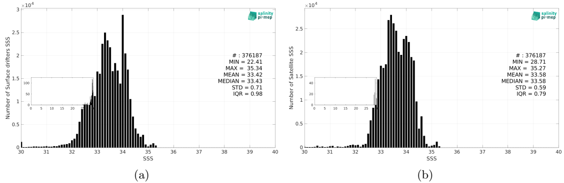
Figure 3: Histograms of SSS from Surface drifters (a) and SMAP SSS L4 OI v3 - Monthly (ESR) (b) considering all match-up pairs per bins of 0.1 over the North Pacific Ocean Pi-MEP region and for the full satellite product period.
