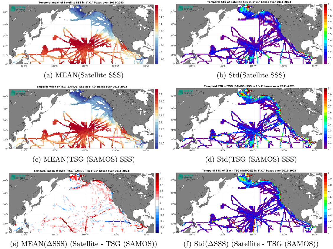
Figure 7: Temporal mean (left) and Std (right) of SSS from SMAP SSS L4 OI v3 - Daily (ESR) (top), TSG (SAMOS) (middle), and of \Delta\text{SSS} (Satellite - TSG (SAMOS)). Only match-up pairs are used to generate these maps.
