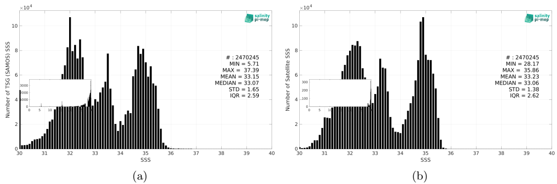
Figure 3: Histograms of SSS from TSG (SAMOS) (a) and SMAP SSS L4 OI v3 - Daily (ESR) (b) considering all match-up pairs per bins of 0.1 over the North Pacific Ocean Pi-MEP region and for the full satellite product period.
