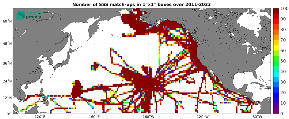
Figure 5: Number of SSS match-ups between TSG (SAMOS) SSS and the SMAP SSS L4 OI v3 - Daily (ESR) SSS product for the North Pacific Ocean Pi-MEP region over 1^\circ \times 1^\circ boxes and for the full satellite product period.
