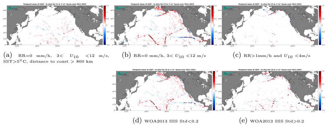
Figure 14: Temporal mean gridded over spatial boxes of size 1^\circ \times 1^\circ of \Delta SSS (SMAP SSS L4 OI v3 - Daily (ESR) - TSG (SAMOS)) for 5 different subdatasets corresponding to: RR=0 mm/h, 3 < U_{10} < 12 m/s, SST > 5°C, distance to coast > 800 km (a), RR=0 mm/h, 3 < U_{10} < 12 m/s (b), RR > 1mm/h and U_{10} < 4 m/s (c), WOA2013 SSS Std < 0.2 (d), WOA2013 SSS Std > 0.2 (e).
