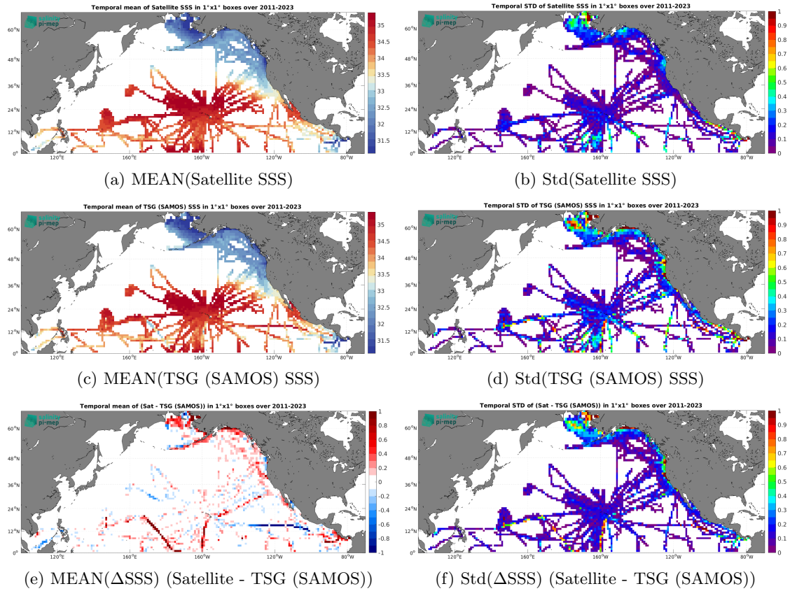
Figure 7: Temporal mean (left) and Std (right) of SSS from SMAP SSS L4 OI v3 - Daily (ESR) (top), TSG (SAMOS) (middle), and of \Delta SSS (Satellite - TSG (SAMOS)). Only match-up pairs are used to generate these maps.
