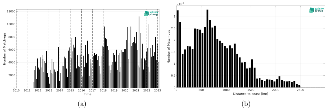
Figure 2: Number of match-ups between TSG (LEGOS-DM) and SMAP SSS L4 OI v3 - Daily (ESR) SSS as a function of time (a) and as function of the distance to coast (b) over the North Pacific Ocean Pi-MEP region and for the full satellite product period.
