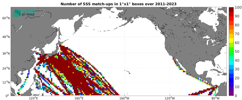
Figure 5: Number of SSS match-ups between TSG (LEGOS-DM) SSS and the SMAP SSS L4 OI v3 - Daily (ESR) SSS product for the North Pacific Ocean Pi-MEP region over 1^\circ \times 1^\circ boxes and for the full satellite product period.
