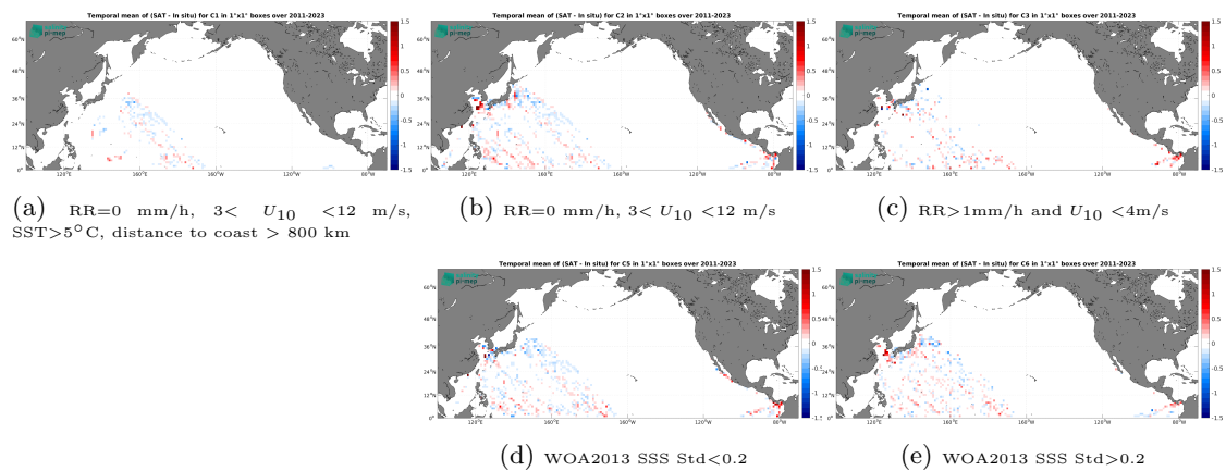
Figure 14: Temporal mean gridded over spatial boxes of size 1^\circ \times 1^\circ of \Delta\text{SSS} (SMAP SSS L4 OI v3 - Daily (ESR) - TSG (LEGOS-DM)) for 5 different subdatasets corresponding to: RR=0 mm/h, 3 < U_{10} < 12 m/s, SST > 5°C, distance to coast > 800 km (a), RR=0 mm/h, 3 < U_{10} < 12 m/s (b), RR > 1 mm/h and U_{10} < 4 m/s (c), WOA2013 SSS Std < 0.2 (d), WOA2013 SSS Std > 0.2 (e).
