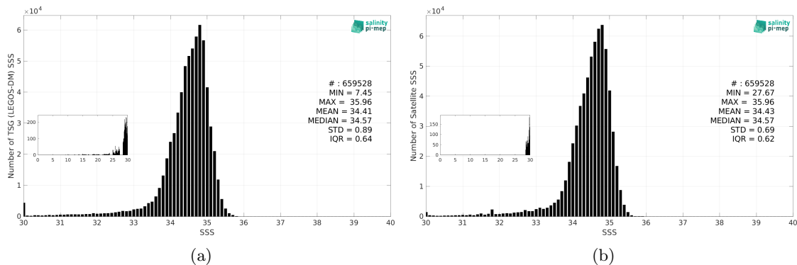
Figure 3: Histograms of SSS from TSG (LEGOS-DM) (a) and SMAP SSS L4 OI v3 - Daily (ESR) (b) considering all match-up pairs per bins of 0.1 over the North Pacific Ocean Pi-MEP region and for the full satellite product period.
