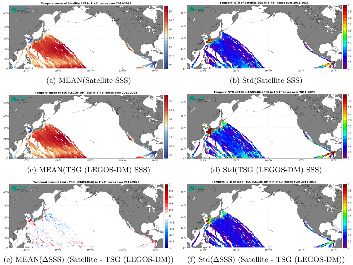
Figure 7: Temporal mean (left) and Std (right) of SSS from SMAP SSS L4 OI v3 - Daily (ESR) (top), TSG (LEGOS-DM) (middle), and of \Delta SSS (Satellite - TSG (LEGOS-DM)). Only match-up pairs are used to generate these maps.
