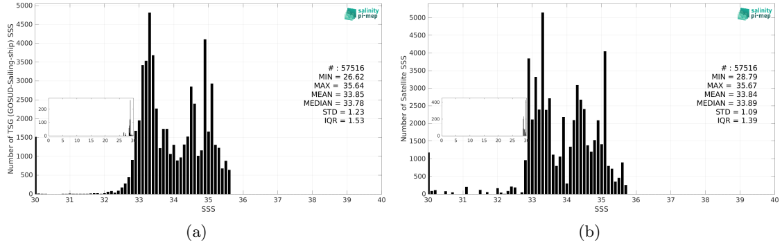
Figure 3: Histograms of SSS from TSG (GOSUD-Sailing-ship) (a) and SMAP SSS L4 OI v3 - Daily (ESR) (b) considering all match-up pairs per bins of 0.1 over the North Pacific Ocean Pi-MEP region and for the full satellite product period.
