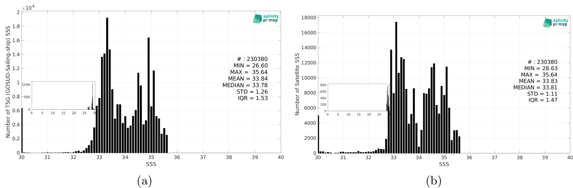
Figure 3: Histograms of SSS from TSG (GOSUD-Sailing-ship) (a) and SMAP SSS L4 OI v3 - Daily (ESR) (b) considering all match-up pairs per bins of 0.1 over the North Pacific Ocean Pi-MEP region and for the full satellite product period.
