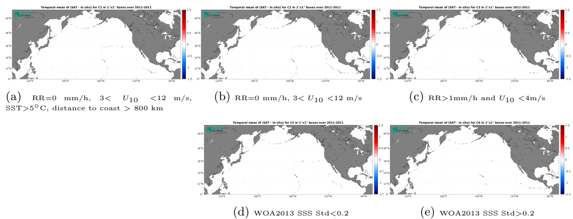
Figure 14: Temporal mean gridded over spatial boxes of size 1^\circ \times 1^\circ of \Delta SSS (SMAP SSS L4 OI v3 - Daily (ESR) - TSG (GOSUD-Sailing-ship)) for 5 different subdatasets corresponding to:RR=0 mm/h, 3 < U_{10} < 12 m/s, SST>5°C, distance to coast > 800 km (a), RR=0 mm/h, 3 < U_{10} < 12 m/s (b), RR>1mm/h and U_{10} < 4 m/s (c), WOA2013 SSS Std<0.2 (d), WOA2013 SSS Std>0.2 (e).
