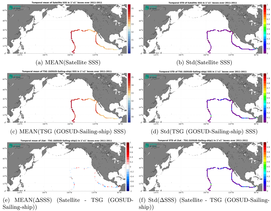
Figure 7: Temporal mean (left) and Std (right) of SSS from SMAP SSS L4 OI v3 - Daily (ESR) (top), TSG (GOSUD-Sailing-ship) (middle), and of \Delta SSS (Satellite - TSG (GOSUD-Sailing-ship)). Only match-up pairs are used to generate these maps.
