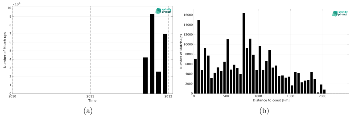
Figure 2: Number of match-ups between TSG (GOSUD-Sailing-ship) and SMAP SSS L4 OI v3 - Daily (ESR) SSS as a function of time (a) and as function of the distance to coast (b) over the North Pacific Ocean Pi-MEP region and for the full satellite product period.
