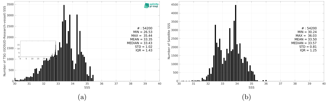
Figure 3: Histograms of SSS from TSG (GOSUD-Research-vessel) (a) and SMAP SSS L4 OI v3 - Daily (ESR) (b) considering all match-up pairs per bins of 0.1 over the North Pacific Ocean Pi-MEP region and for the full satellite product period.
