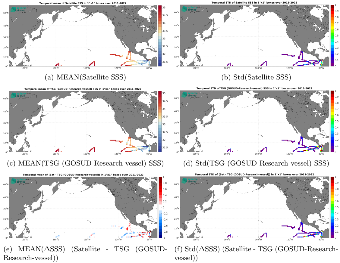
Figure 7: Temporal mean (left) and Std (right) of SSS from SMAP SSS L4 OI v3 - Daily (ESR) (top), TSG (GOSUD-Research-vessel) (middle), and of \Delta SSS (Satellite - TSG (GOSUD-Research-vessel)). Only match-up pairs are used to generate these maps.
