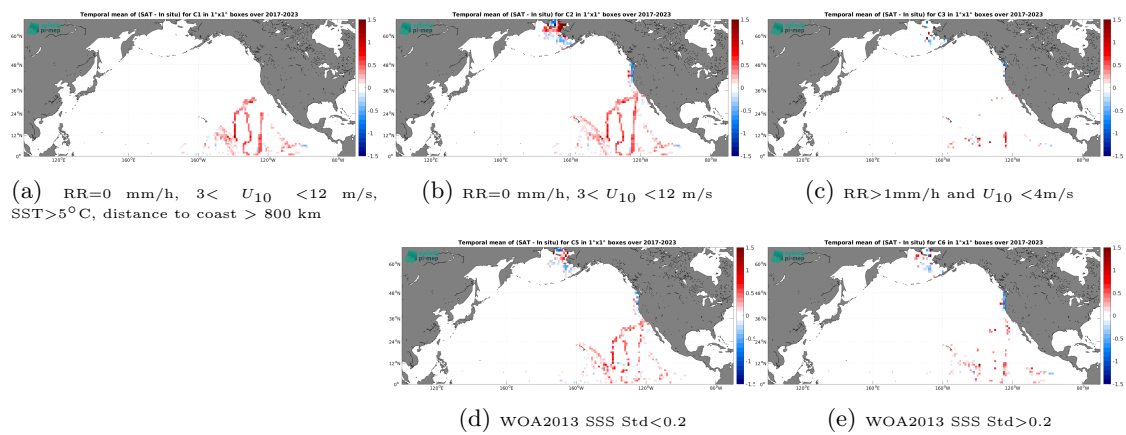
Figure 14: Temporal mean gridded over spatial boxes of size 1^\circ \times 1^\circ of \Delta SSS (SMAP SSS L4 OI v3 - Daily (ESR) - Saildrone) for 5 different subdatasets corresponding to: RR=0 mm/h, 3 < U_{10} < 12 m/s, SST > 5°C, distance to coast > 800 km (a), RR=0 mm/h, 3 < U_{10} < 12 m/s (b), RR > 1mm/h and U_{10} < 4 m/s (c), WOA2013 SSS Std < 0.2 (d), WOA2013 SSS Std > 0.2 (e).
