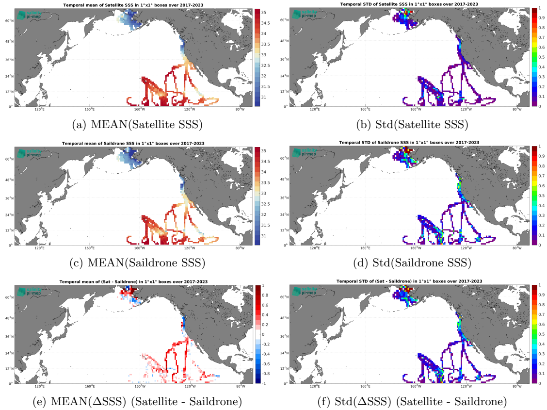
Figure 7: Temporal mean (left) and Std (right) of SSS from SMAP SSS L4 OI v3 - Daily (ESR) (top), Saildrone (middle), and of \Delta SSS (Satellite - Saildrone). Only match-up pairs are used to generate these maps.
