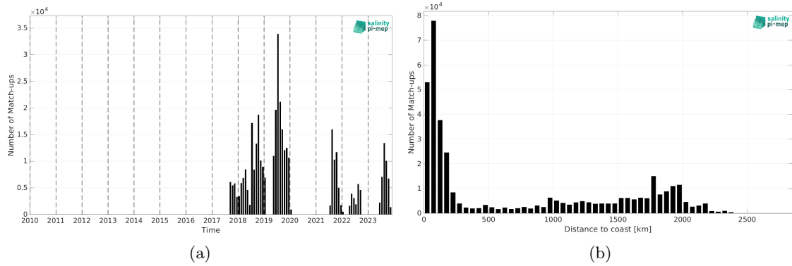
Figure 2: Number of match-ups between Saildrone and SMAP SSS L4 OI v3 - Daily (ESR) SSS as a function of time (a) and as function of the distance to coast (b) over the North Pacific Ocean Pi-MEP region and for the full satellite product period.
