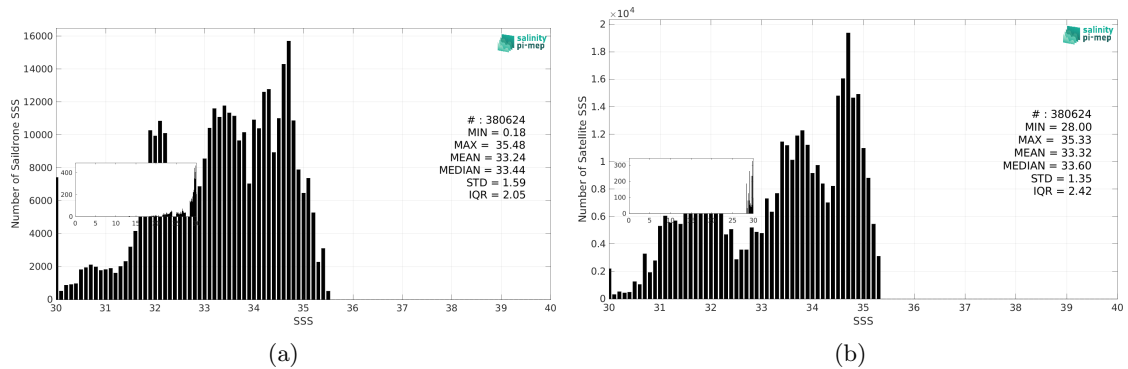
Figure 3: Histograms of SSS from Saildrone (a) and SMAP SSS L4 OI v3 - Daily (ESR) (b) considering all match-up pairs per bins of 0.1 over the North Pacific Ocean Pi-MEP region and for the full satellite product period.
