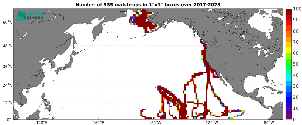
Figure 5: Number of SSS match-ups between Saildrone SSS and the SMAP SSS L4 OI v3 - Daily (ESR) SSS product for the North Pacific Ocean Pi-MEP region over 1^\circ \times 1^\circ boxes and for the full satellite product period.
