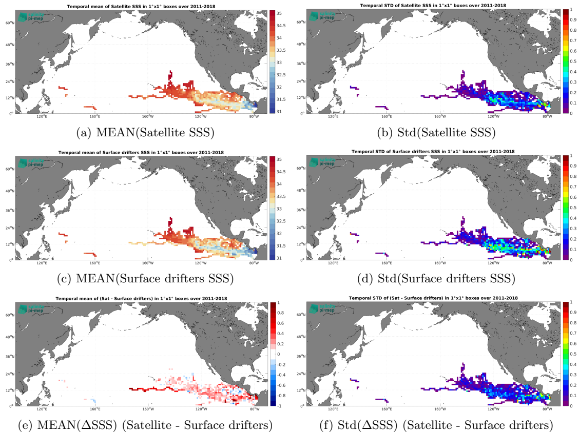
Figure 6: Temporal mean (left) and Std (right) of SSS from SMAP SSS L4 OI v3 - Daily (ESR) (top), Surface drifters (middle), and of \Delta SSS (Satellite - Surface drifters). Only match-up pairs are used to generate these maps.
