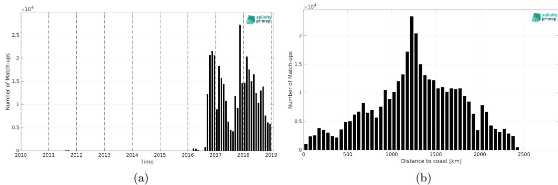
Figure 2: Number of match-ups between Surface drifters and SMAP SSS L4 OI v3 - Daily (ESR) SSS as a function of time (a) and as function of the distance to coast (b) over the North Pacific Ocean Pi-MEP region and for the full satellite product period.
