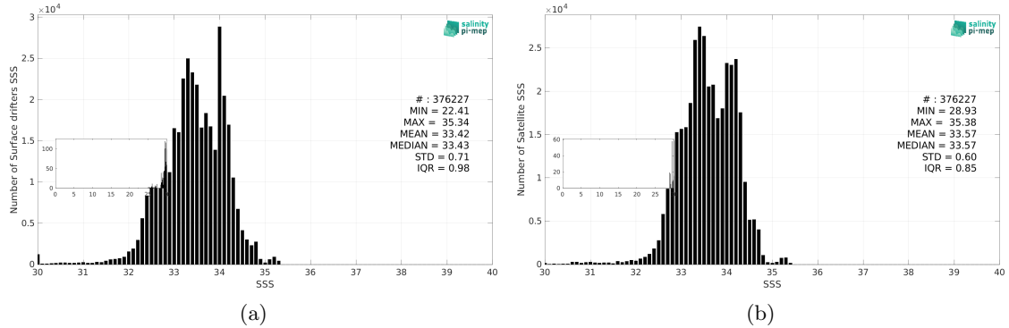
Figure 3: Histograms of SSS from Surface drifters (a) and SMAP SSS L4 OI v3 - Daily (ESR) (b) considering all match-up pairs per bins of 0.1 over the North Pacific Ocean Pi-MEP region and for the full satellite product period.
