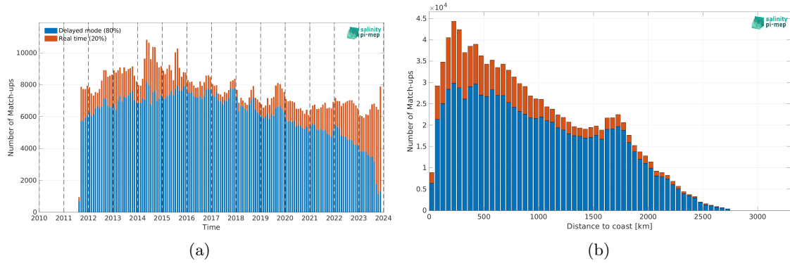
Figure 2: Number of match-ups between Argo and SMAP SSS L4 OI v3 - Daily (ESR) SSS as a function of time (a) and as function of the distance to coast (b) over the North Pacific Ocean Pi-MEP region and for the full satellite product period.
