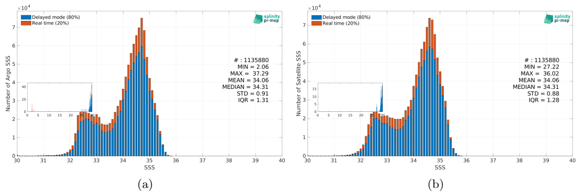
Figure 3: Histograms of SSS from Argo (a) and SMAP SSS L4 OI v3 - Daily (ESR) (b) considering all match-up pairs per bins of 0.1 over the North Pacific Ocean Pi-MEP region and for the full satellite product period.
