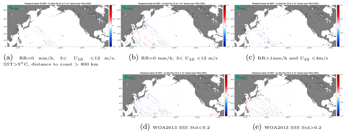
Figure 12: Temporal mean gridded over spatial boxes of size 1^\circ \times 1^\circ of \Delta SSS (SMAP SSS L4 OI v2 - 7 Days (ESR) - TSG (LEGOS-DM)) for 5 different subdatasets corresponding to: RR=0 mm/h, 3 < U_{10} < 12 m/s, SST > 5^\circ C , distance to coast > 800 km (a), RR=0 mm/h, 3 < U_{10} < 12 m/s (b), RR > 1 mm/h and U_{10} < 4 m/s (c), WOA2013 SSS Std < 0.2 (d), WOA2013 SSS Std > 0.2 (e).
