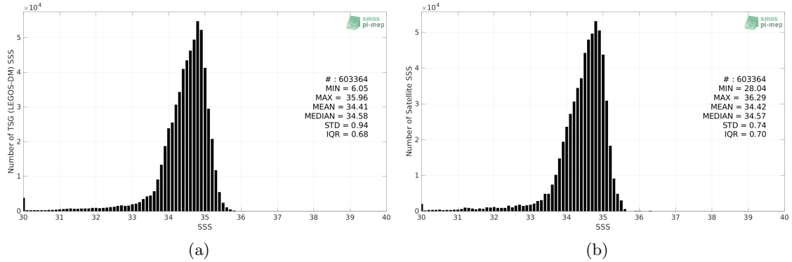
Figure 2: Histograms of SSS from TSG (LEGOS-DM) (a) and SMAP SSS L4 OI v2 - 7 Days (ESR) (b) considering all match-up pairs per bins of 0.1 over the North Pacific Ocean Pi-MEP region and for the full satellite product period.
