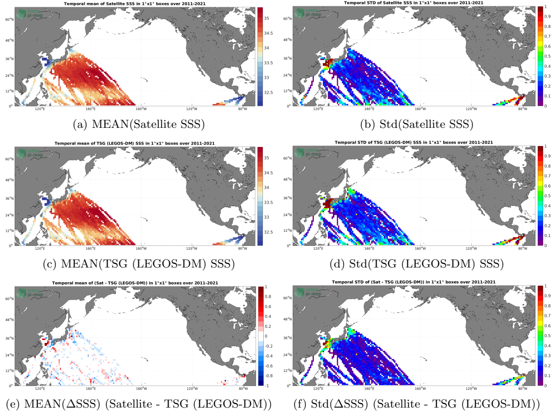
Figure 6: Temporal mean (left) and Std (right) of SSS from SMAP SSS L4 OI v2 - 7 Days (ESR) (top), TSG (LEGOS-DM) (middle), and of \Delta\text{SSS} (Satellite - TSG (LEGOS-DM)). Only match-up pairs are used to generate these maps.
