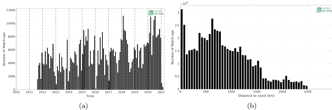
Figure 1: Number of match-ups between TSG (LEGOS-DM) and SMAP SSS L4 OI v2 - 7 Days (ESR) SSS as a function of time (a) and as function of the distance to coast (b) over the North Pacific Ocean Pi-MEP region and for the full satellite product period.
