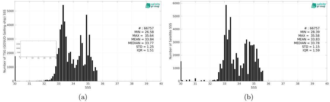
Figure 2: Histograms of SSS from TSG (GOSUD-Sailing-ship) (a) and SMAP SSS L4 OI v2 - 7 Days (ESR) (b) considering all match-up pairs per bins of 0.1 over the North Pacific Ocean Pi-MEP region and for the full satellite product period.
