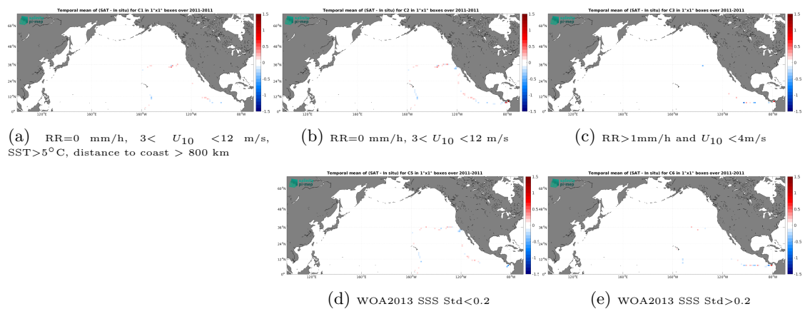
Figure 12: Temporal mean gridded over spatial boxes of size 1^\circ \times 1^\circ of \Delta\text{SSS} (SMAP SSS L4 OI v2 - 7 Days (ESR) - TSG (GOSUD-Sailing-ship)) for 5 different subdatasets corresponding to:RR=0 mm/h, 3 < U_{10} < 12 m/s, SST>5°C, distance to coast > 800 km (a), RR=0 mm/h, 3 < U_{10} < 12 m/s (b), RR>1mm/h and U_{10} < 4 m/s (c), WOA2013 SSS Std<0.2 (d), WOA2013 SSS Std>0.2 (e).
